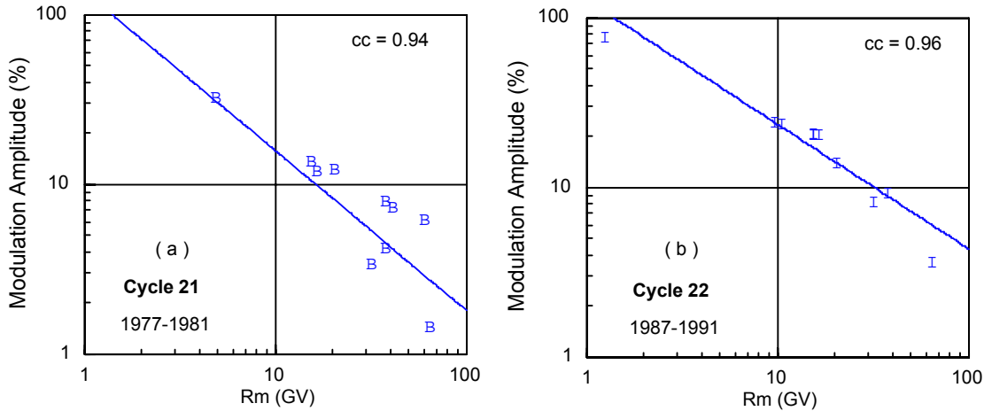
Figure 1 a,b. Amplitude (%) of modulation versus Rm (GV) for the detectors are plotted on a log-log scale. The diagonal lines represent power law fits to the data for two adjacent solar cycles (21, 22).
