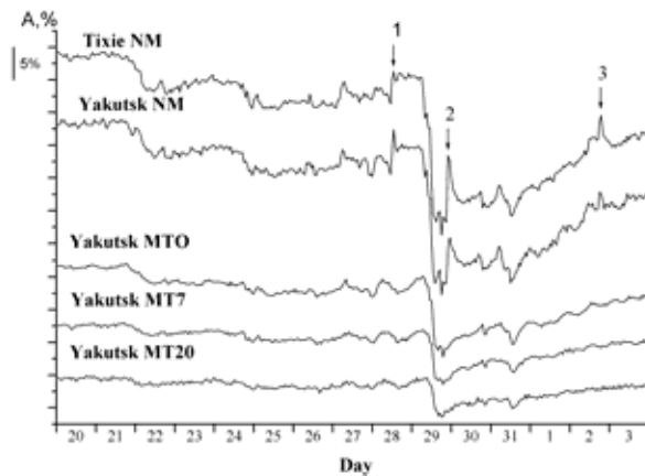
Figure 1. Temporal change of the cosmic ray intensity in October-November 2003 by data of the neutron monitors at Tixie Bay and Yakutsk stations, muon 0,7, 20 m w.e. telescopes at the Yakutsk station. The increases of solar energetic particles are marked by arrows and numbers.
