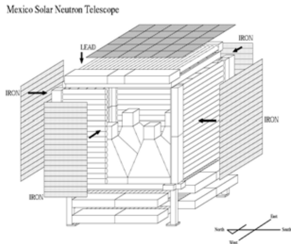
Figure 2. Schematic view of the SNT at Sierra Negra Volcano. Four 1\text{m}^2 scintillators are shielded by anticoincidence system. On the top of the telescope, a 5 cm thick lead plate is installed to convert background photons in e^-e^+ pairs. Below of the scintillator, four layers of PRC array are used to identify the arrival directions of neutrons.
