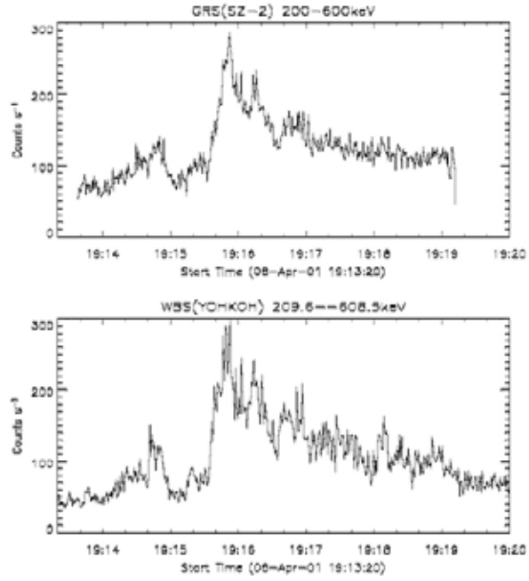
Figure5 light curve of SF010406, SZ2/GD(top), and Yokkoh (down) observation, X5.6 flare
