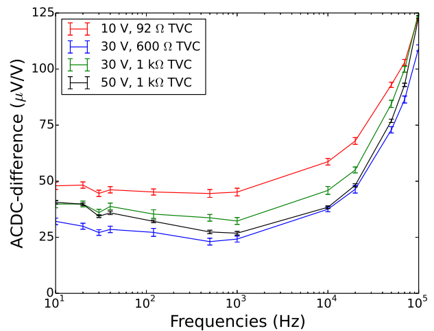
Fig. 8. Resulting ac-dc difference for the divider and buffer combination from 10 Hz up to the maximum capability of the calibrator. Red curve contains the measurements for 10 V, blue curve contains the measurements for 30 V, and black curve contains the measurements for 50 V. The green curve contains the measurements for 30 V, by using the references used for 50 V.
