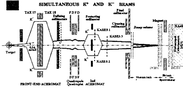
Figure 1: The NA48/2 beam line and detector. Not to scale.
