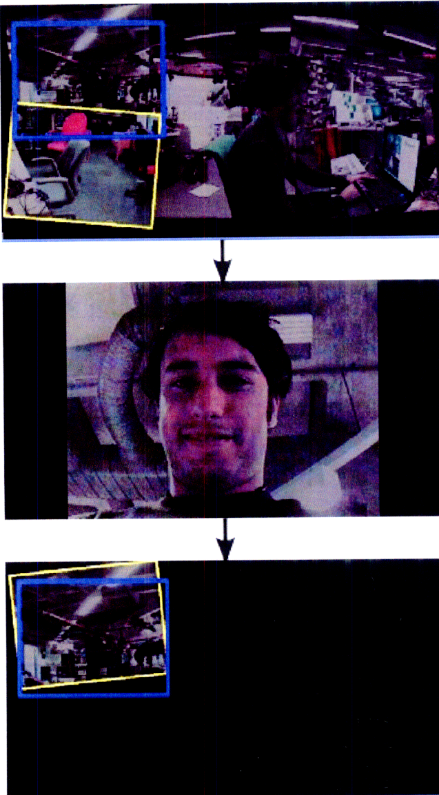
Figure 19: A time-sequence of what happens when the robot is picked up and moved to a new location. The first image illustrates the stale panorama before the robot has been picked up, the second is when the robot is in motion (i.e. being carried), and the third image illustrates what the panorama looks like when no motion is detected by the IMU. In the third image, the stale panorama is cleared out since the old panorama no longer reflects the new remote environment. A new stale panorama would then be subsequently built.
