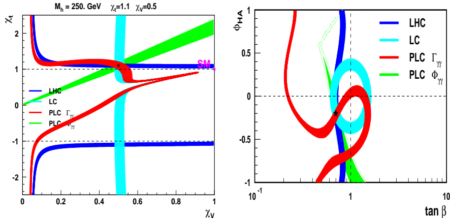
Fig. 6. The left panel shows the synergy between the LHC/ILC and the PLC in precise determination of the Higgs Boson couplings in a general 2 Higgs Doublet Model [16]. The star at (1,1) indicates the SM point and the 'star' at the centre of the plot corresponds to a particular set of parameters for the general 2HDM for which the light Higgs has a SM-like phenomenology. The plot in the right panel shows an example of the same synergy for the case of the Higgs Boson couplings in a CP violating 2HDM [17]. The plot shows that the measurements at all the three colliders will be needed to determine conclusively whether the CP-violating phase is nonzero.
