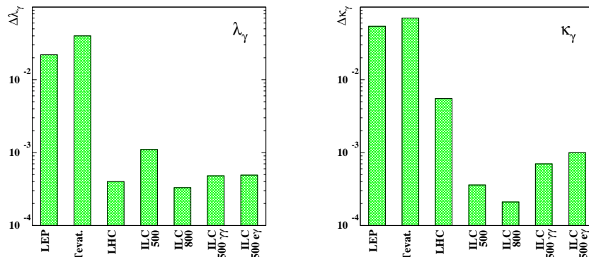
Fig. 7. A compilation of the reach of various colliders for the anomalous couplings of the photon [18].
