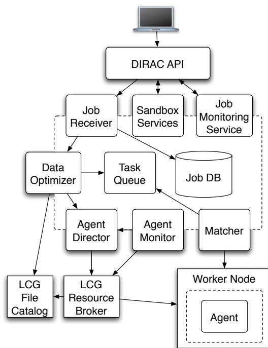
Figure 3 Outline of the DIRAC Workload Management System.
