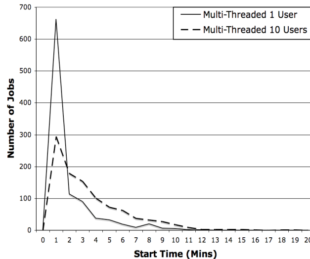
Figure 7 Comparison of the effect of number of users on the start time of jobs.
