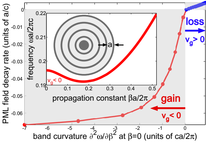
FIG. 1: Field decay rate within the PML vs. curvature of the dispersion relation at \beta = 0 , showing onset of gain for v_g < 0 and loss for v_g > 0 . Inset . Dispersion relation (of the first TE band) with v_g < 0 region at \beta = 0 , and cross-section of the Bragg fiber.
