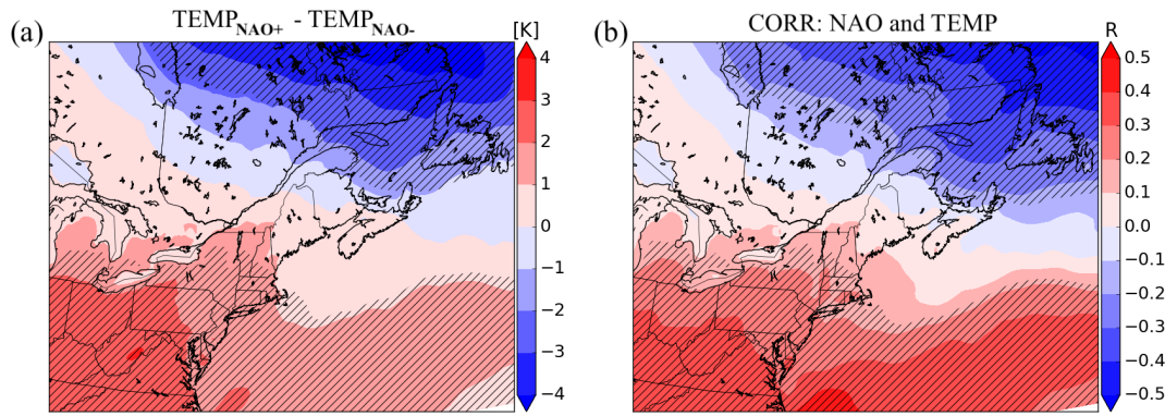
Figure 6. (a) Difference between average temperature during positive NAO and negative NAO months (40-month composites, first and fourth quartiles) in winter (DJFM); positive values mean warmer temperatures during high NAO. (b) Correlation coefficients between monthly temperature and monthly NAOI. Hatched areas represent statistically significant values at the 0.05 level.
