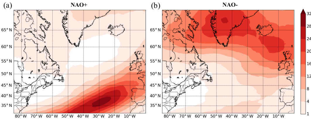
Figure 10. Blocking frequency averaged over (a) positive NAO months and (b) negative NAO months (40-month composites, first and fourth quartiles in winter (DJFM)).
