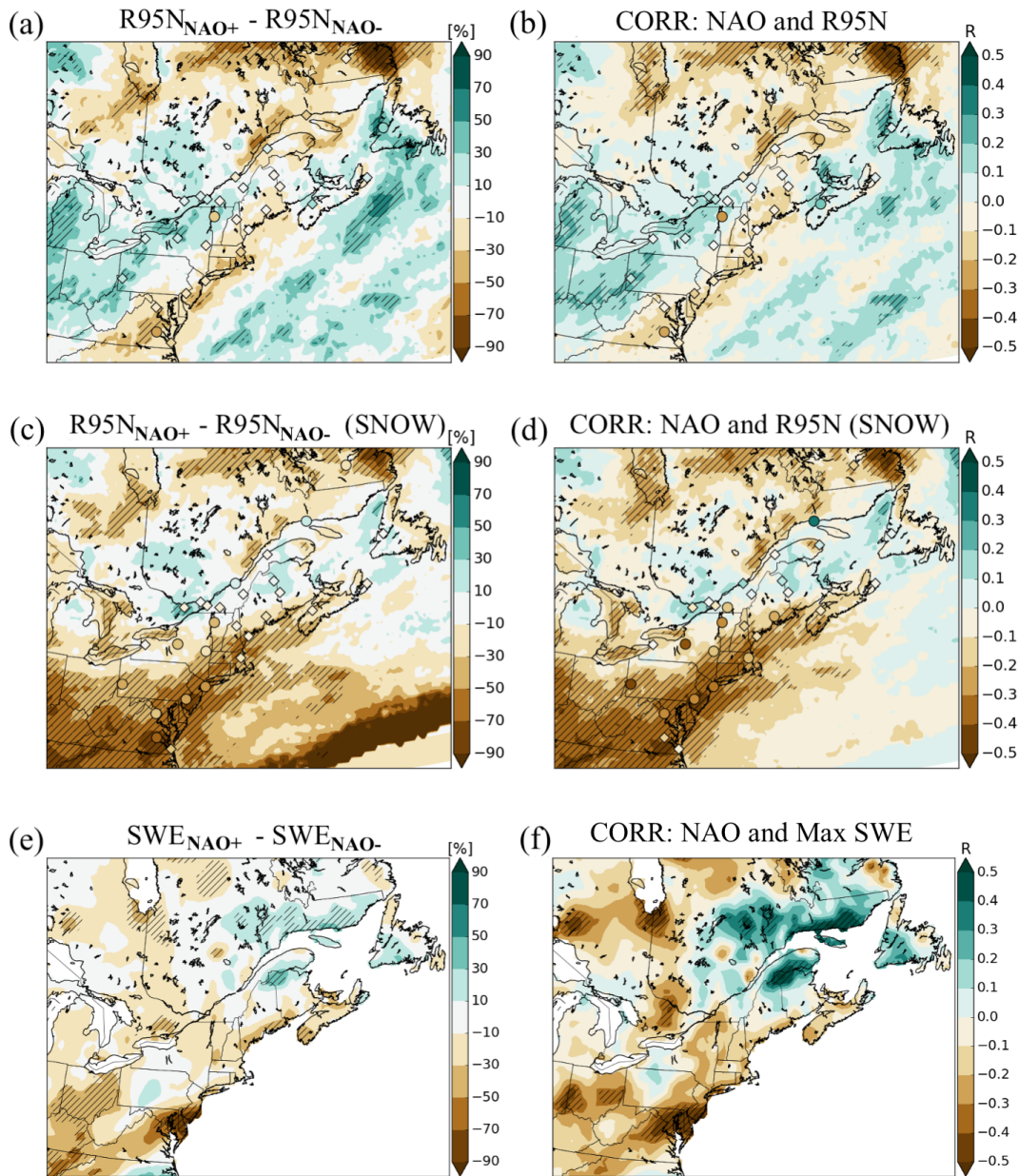
Figure 5. (a) Relative difference between the number of heavy precipitation days (above 95th percentile of daily precipitation, R95N) during positive NAO and negative NAO months (40-month composites, first and fourth quartiles) in winter (DJFM). (b) Correlation coefficients between number of heavy precipitation days and monthly NAOI. Hatched areas represent statistically significant values at the 0.05 level. Shaded circles represent station-based correlation coefficients that are statistically significant at the 0.05 level, and diamonds represent values that are not statistically significant. (c, d) As in panels (a) and (b) but for the relationship between monthly NAO and the number of heavy snowfall days (above 95th percentile of daily snowfall). (e, f) As in panels (a) and (b) but for the relationship between cold season averaged NAO and annual maximum snowpack depth.
