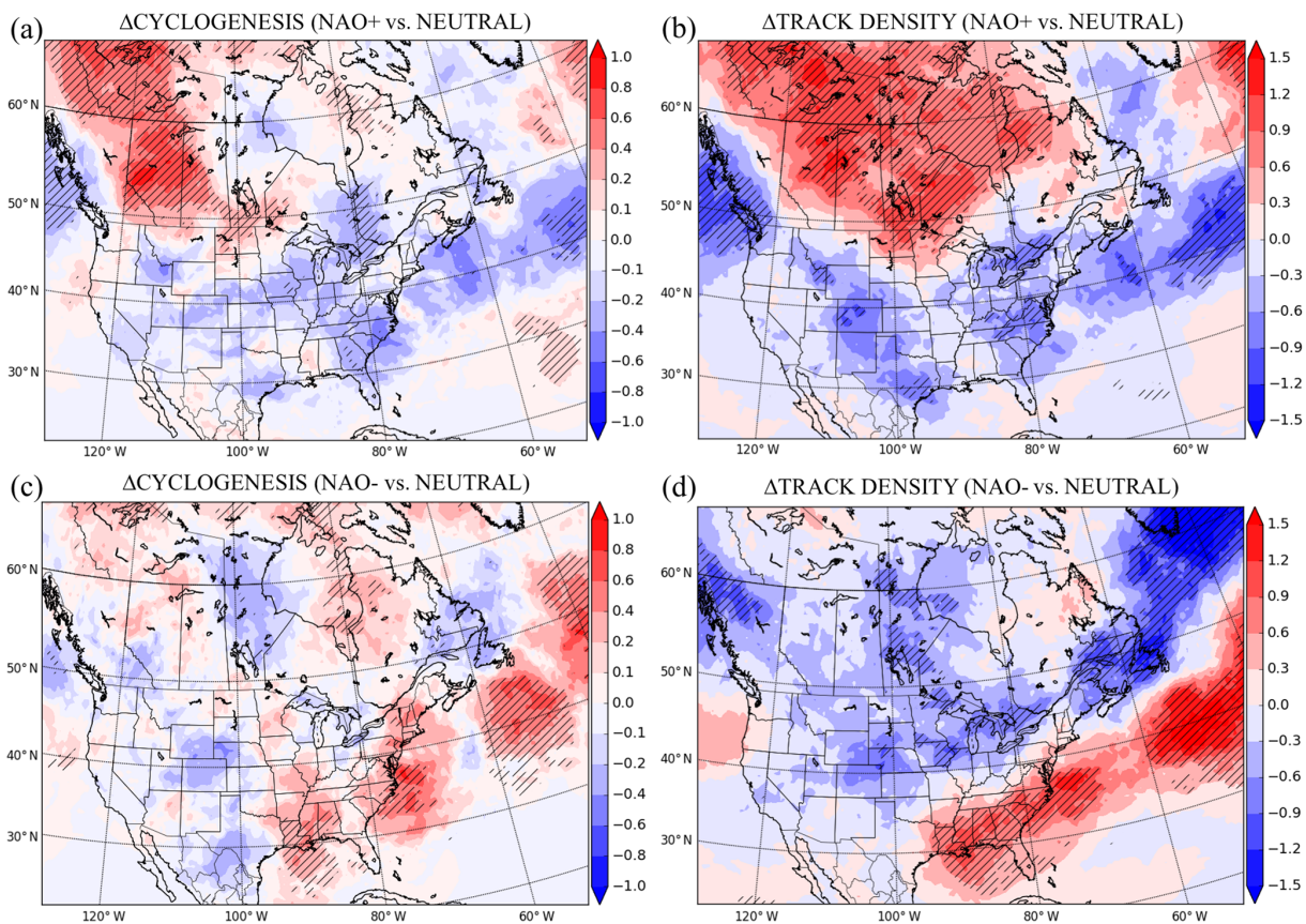
Figure 7. Anomalies of (a, c) cyclogenesis and (b, d) track density (cyclone/month per area of 1000 km 2 ) over the course of (a, b) positive NAO and (c, d) negative NAO months (40-month composites, first and fourth quartiles) in winter (DJFM); positive values mean higher cyclone occurrence. Anomalies are calculated in relation to an average neutral NAO month. Hatched areas represent statistically significant values at the 0.05 level.
