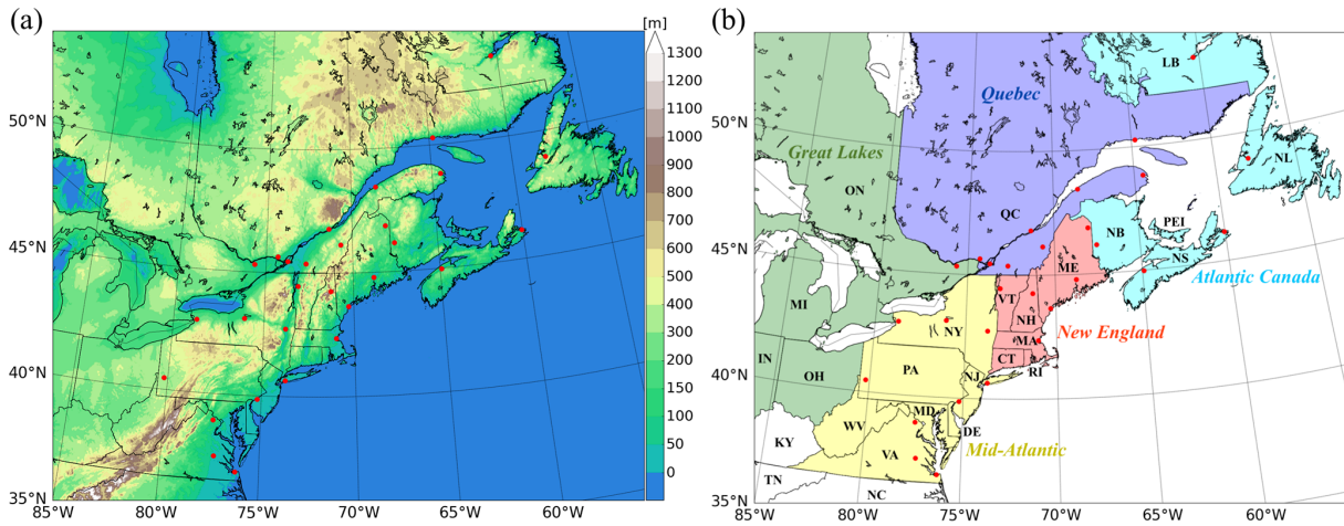
Figure 2. (a) Map of the domain of interest with elevation included. The elevation data shown are ETOPO1 1 Arc-Minute Global Relief (retrieved from https://www.ngdc.noaa.gov/mgg/global/ , last access: 24 November 2020; Amante and Eakins, 2009). Red dots represent the locations of the weather stations used in the study as data validation. (b) Map of the domain of interest separated by main geographical regions, with the abbreviations of Canadian provinces and US states included.
