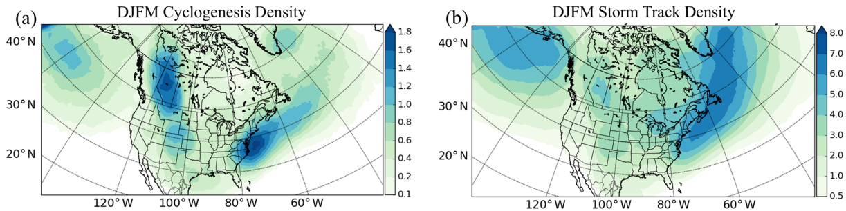
Figure 3. ERA5 average cool-season (December to March) (a) cyclogenesis density and (b) storm track density over the 1979–2018 period. The units are number of cyclones per month per area of 1000 km 2 .
