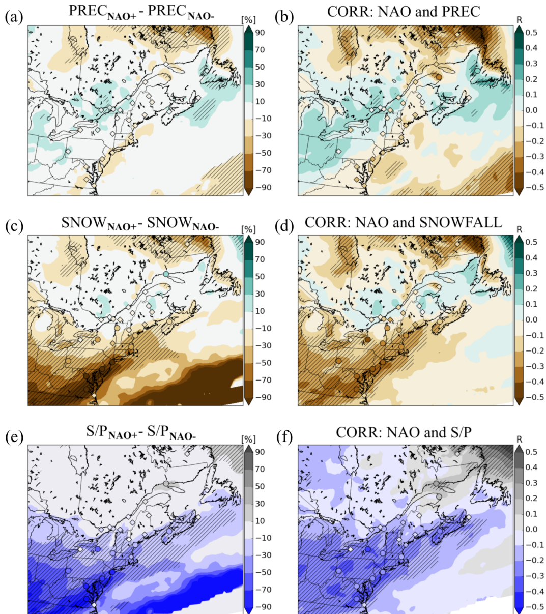
Figure 4. (a) Relative difference between average precipitation during positive NAO and negative NAO months (40-month composites, first and fourth quartiles) in winter (DJFM); positive values mean more precipitation during high NAO. (b) Correlation coefficients between monthly precipitation and monthly NAOI. Hatched areas represent statistically significant values at the 0.05 level. Shaded circles represent station-based correlation coefficients that are statistically significant at the 0.05 level, and diamonds represent values that are not statistically significant. (c, d) As in panels (a) and (b) but for the relationship between monthly NAO and snowfall. (e, f) As in panels (a) and (b) but for the relationship between monthly NAO and S/P .
