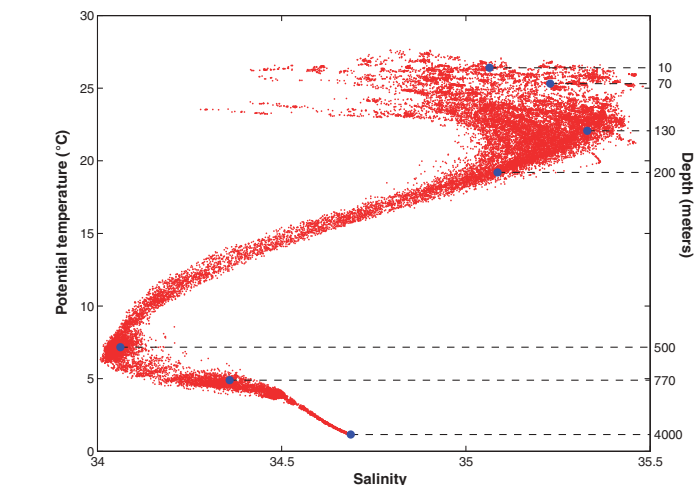
Fig. 1. Temperature versus salinity (T-S) relations for the North Pacific Subtropical Gyre at station ALOHA (22°45'N, 158°W). The blue circles indicate the positions, in T-S “hyospace” of the seven water samples analyzed in this study. The data envelope shows the temperature and salinity conditions observed during the period October 1988 to December 2004 emphasizing both the temporal variability of near-surface waters and the relative constancy of deep waters.
