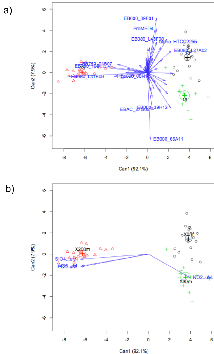
Figure 6. Canonical discriminant (c.d.) analysis of Monterey Bay sample (0m \circ , 30m + , and 200m \triangle ) array data, with parameter correlations to c.d. axes indicated by vector length and direction. (a) Genotype abundance correlations to c.d. axes; the distribution of particular taxa drive the differentiation of depths. (b) Nutrient correlations to c.d. axes; nutrients are dramatically different between the three depths, and this strong difference is recapitulated in the correlations to c.d. axes.
