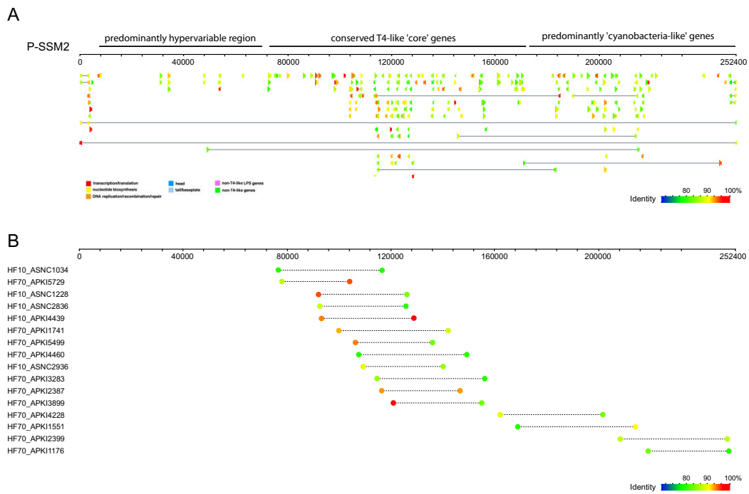
fig S12. Alignment of cyanophage fosmid-mate pairs along a fully sequenced cyanophage genome. fig S12A. Cyanophage-like fosmid end sequences were compared to the complete genome of cyanophage P-SSM-2 by blastn analyses at an expectation cutoff of 1 \times 10^{-3} . All sequences matching at similarities > 80\% identity are shown. Colors indicate the level of sequence similarity. Lines split single sequences that match the genome at high similarity in different regions across the sequence. fig S12B. Selected fosmids that matched P-SSM-2 with high sequence similarity on both fosmid ends were aligned to the whole phage genome sequence. Colors indicate the level of sequence similarity.
