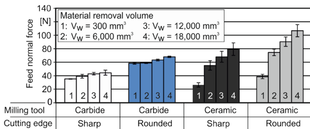
Fig. 8 Feed normal forces after different material removal volumes while machining with ceramic and cemented carbide end mills with sharp and rounded cutting edge
