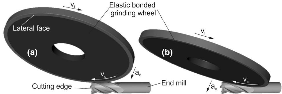
Fig. 2 Cutting edge preparation process at different stages of feed motion while down grinding
