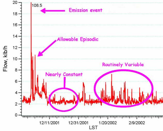
Figure 1. Components of mass flow rates to a flare at an industrial facility in the HG area: nearly constant, routinely variable, allowable episodic, and emission event in order of magnitude (Webster et al., 2007).
