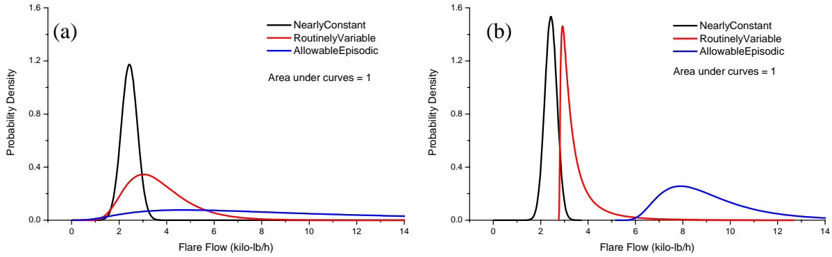
Figure 2. PDFs for each component of emissions from the flare in Figure 1 in (a) the original version of the stochastic inventory generator (Webster et al., 2007); f(x;\mu;\sigma) = \frac{e^{-(\ln x - \mu)^2 / (2\sigma^2)}}{x\sigma\sqrt{2\pi}} for routinely variable and allowable episodic components and (b) the updated version of the stochastic inventory generator (Webster, 2007); f(x;\mu;\sigma) = \frac{e^{-(\ln(x - shift) - \mu)^2 / (2\sigma^2)}}{(x - shift)\sigma\sqrt{2\pi}} for routinely variable and allowable episodic components.
