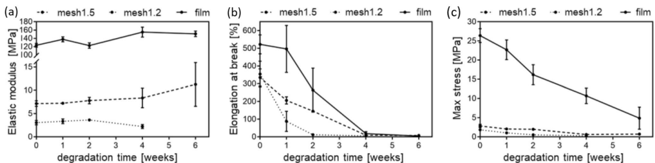
Fig. 4 Changes in mechanical properties at 37 °C of hydrolytically partially degraded PEEU. a Elastic modulus, b elongation at break, and c maximum stress of specimens over time during degradation. n \geq 4
