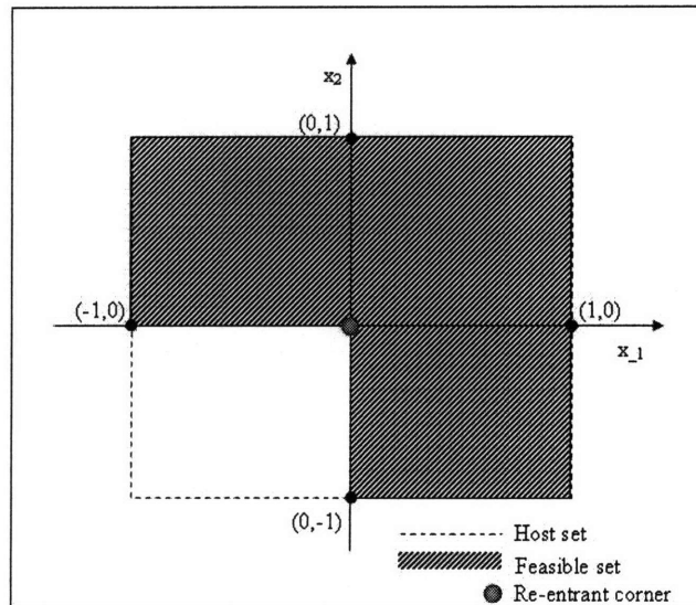
Figure 4-3: Re-entrant Corner Points in GSIP
