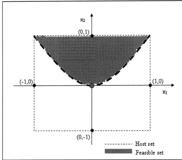
Figure 4-2: Non-closedness of the Feasible Set in GSIP
