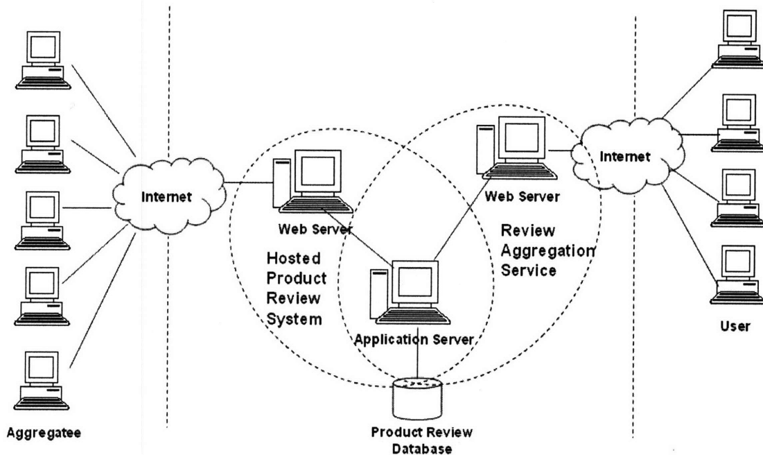
Figure 5-3: Hosted Solution Architecture
