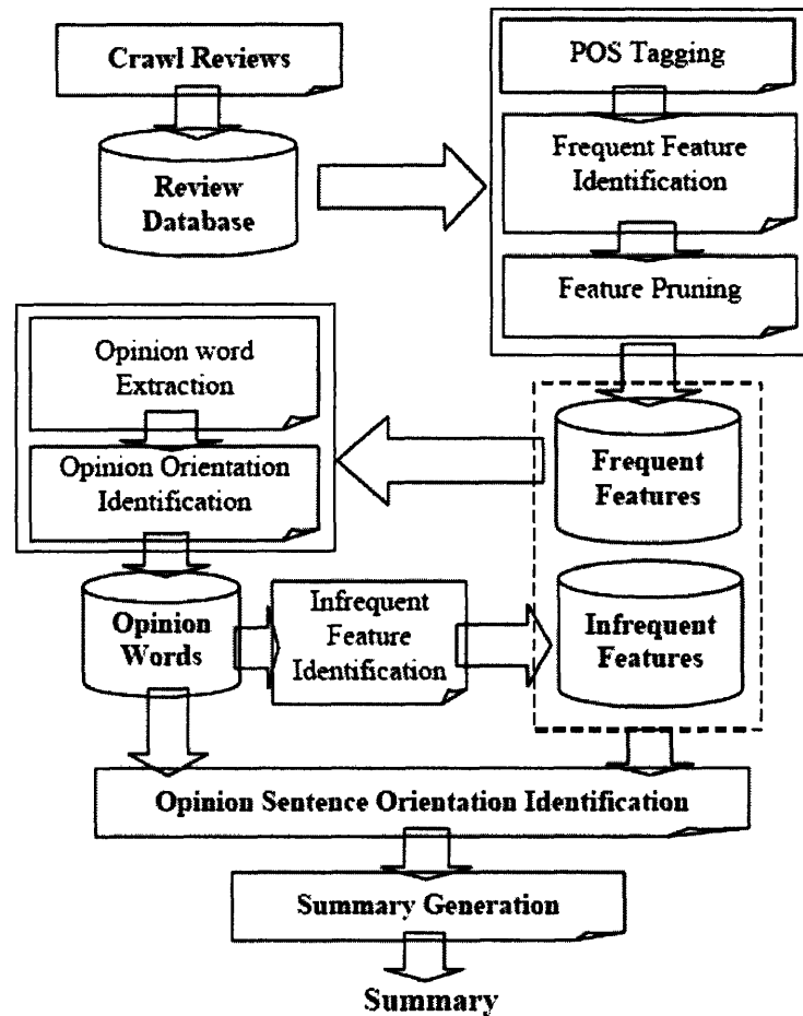
Figure 5-2: Operational Sequence of Feature-based Sentiment Analysis (Source: Hu and Liu, 2004)
