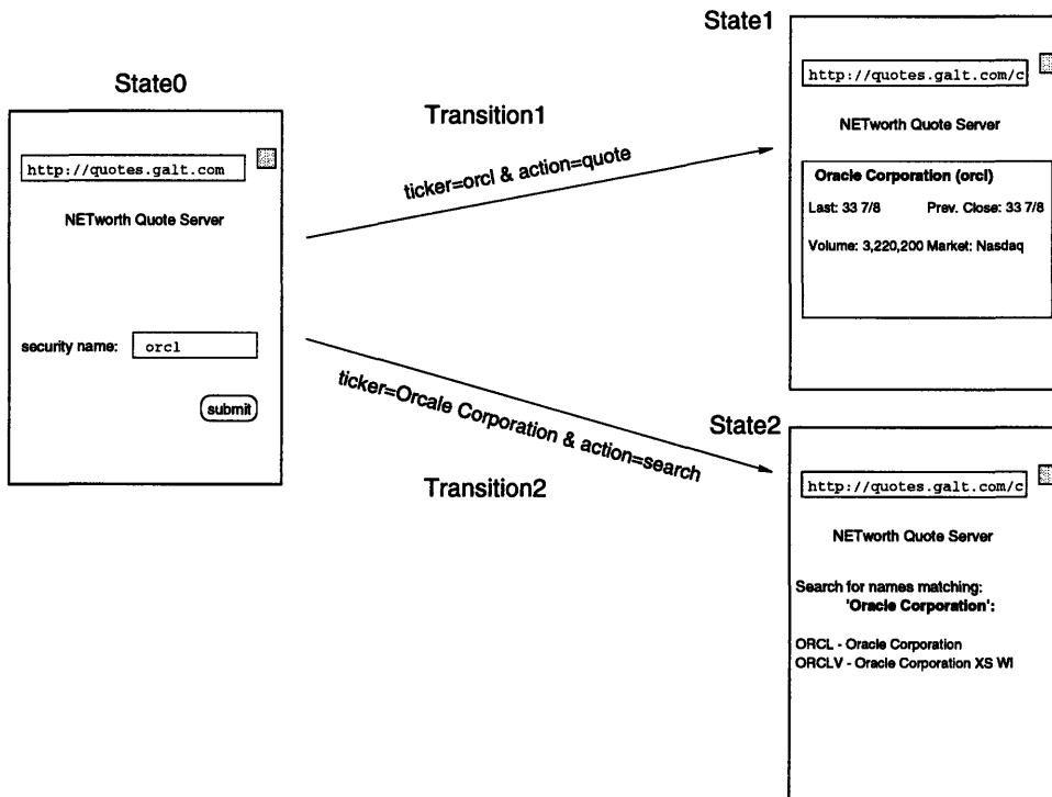
Figure 3-3: State transition diagram for Networth quotes server.
