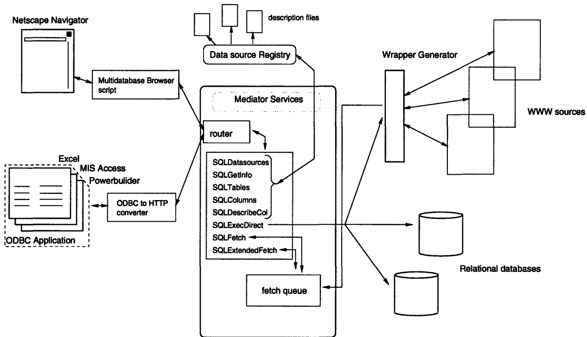
Figure 3-1: COIN Architecture.
