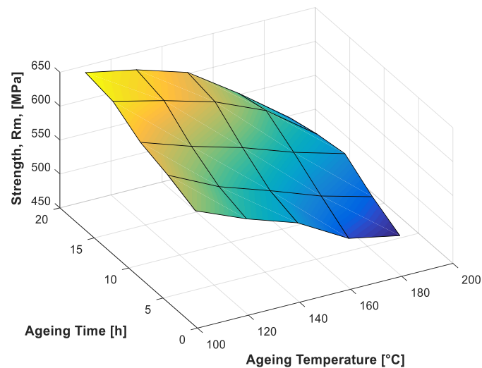
Fig. 2. Variability in breaking resistance of studied alloy with aging time and temperature for \varepsilon = 30\%
