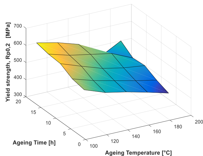
Fig. 3. Variability in flow resistance of studied alloy with time and temperature of aging for \varepsilon = 30\%
