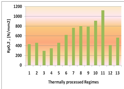
Fig. 3. Variation of the yield point ( R_{p0,2} ) values according to experimental processing regimes
