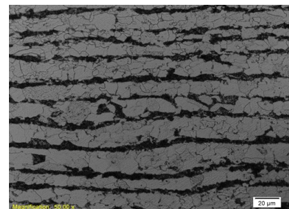
Fig. 8. Perlite distributed in strings and oriented in the direction of deformation (nital attack 3% X500)
