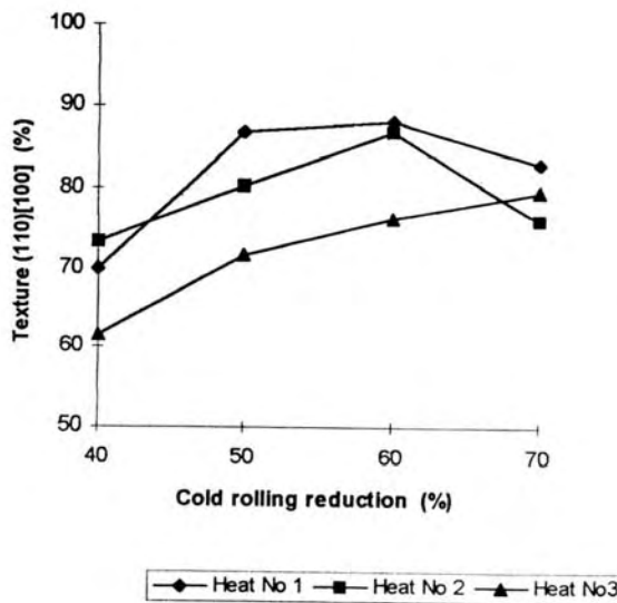
Fig. 2. The influence of the cold rolling reduction ratio on texture (110)[100].
