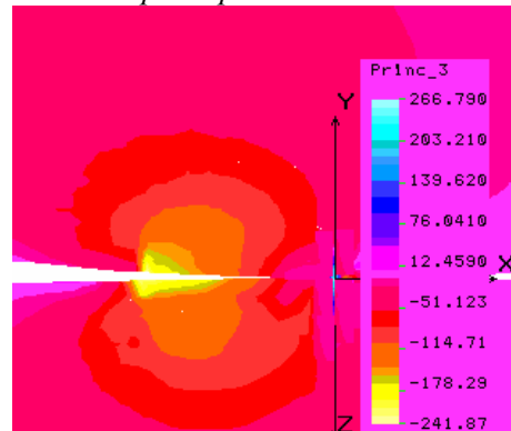
Fig. 13b. Case 2 ( \mu=0.075 ) Phase F_A4 principal stress \sigma_3
