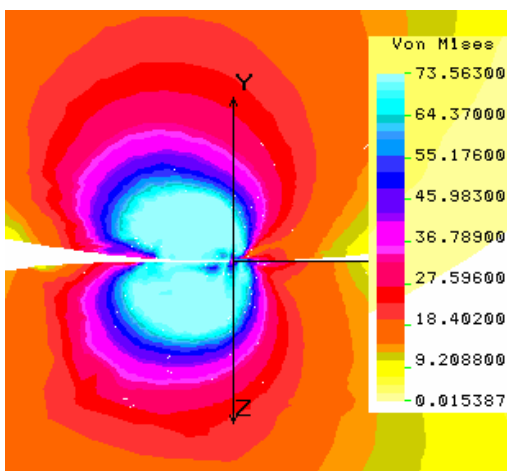
Fig. 8a. Case 1 ( \mu=0.1 ) Phase A5 principal stress \sigma_3
