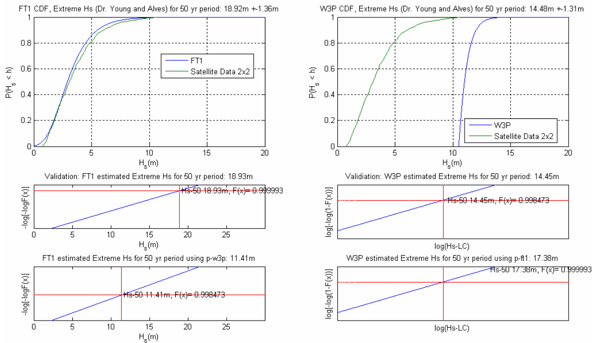
Figure 3.10: H_s prediction comparison, 4 deg x 4 deg grid size, 50 yr return period ( 43^\circ \text{N} , 163^\circ \text{E} )
