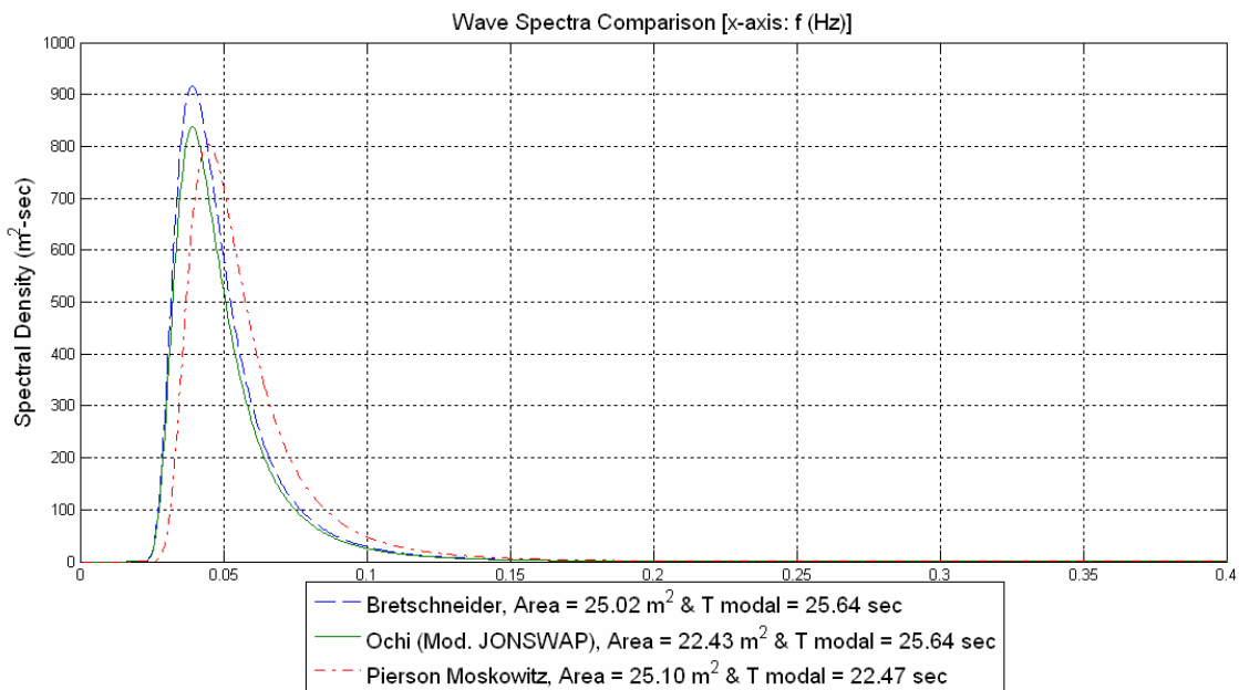
Figure 3.16: Wave amplitude spectra comparison ( T_m prediction using FT1), 2 deg x 2 deg grid size, 50 yr return period, H_s = 21.03\text{m} , T_m = 19.73 \text{ sec} ( 43^\circ \text{ N} , 163^\circ \text{ E} )
