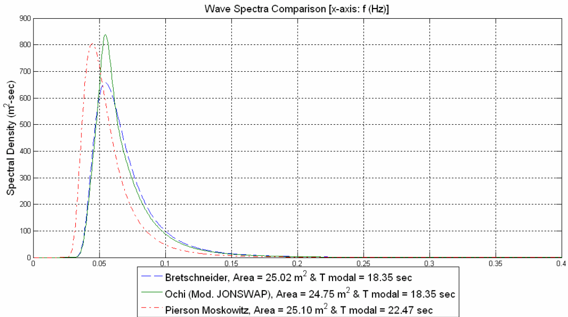
Figure 3.15: Wave amplitude spectra comparison ( T_m prediction using W2P), 2 deg x 2 deg grid size, 50 yr return period, H_s = 20.01\text{m} , T_m = 14.14 \text{ sec} ( 43^\circ \text{ N} , 163^\circ \text{ E} )
