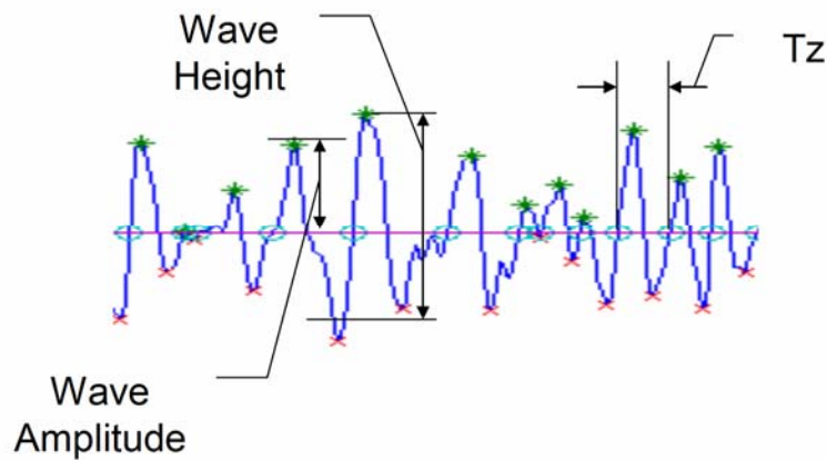
Figure 3.18: Wave parameters
