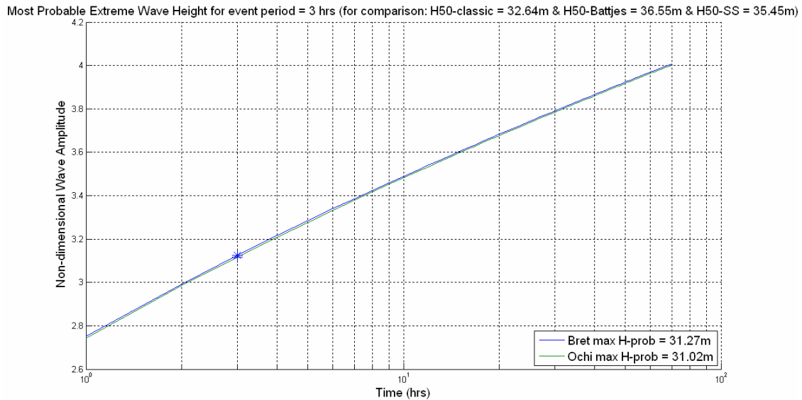
Figure 3.14: Extreme wave amplitude (crest-to-mean) prediction based on short term order statistics (T m estimated using W2P), extreme H s from 2 deg x 2 deg grid size, 50 yr return period, H s = 20.01 m, T m = 14.14 sec (43° N, 163° E)
