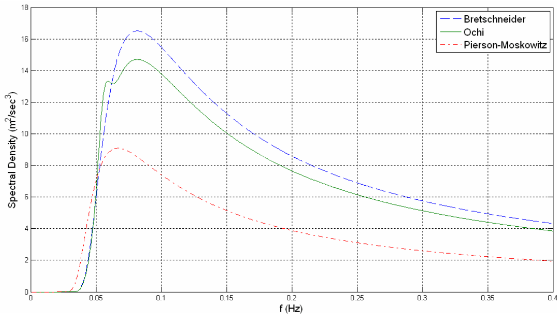
Figure 3.23: Wave vertical acceleration spectra comparison ( T_m prediction using W2P), 2 deg x 2 deg grid size, 50 yr return period, H_s = 20.01\text{m} , T_m = 14.14\text{ sec} ( 43^\circ\text{ N} , 163^\circ\text{ E} )
