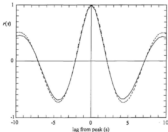
Figure 5.4: The continuous line is the normalized average time history of the wave with the highest crest in each of 1000 random simulations. The dashed line is the theoretical autocorrelation function. The spectrum is JONSWAP with f_m = 0.1 Hz (modal frequency) [35]
