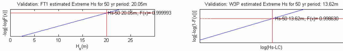
Figure 3.8: FT1/IDM vs. W3P/POT (43° N, 163° E)
