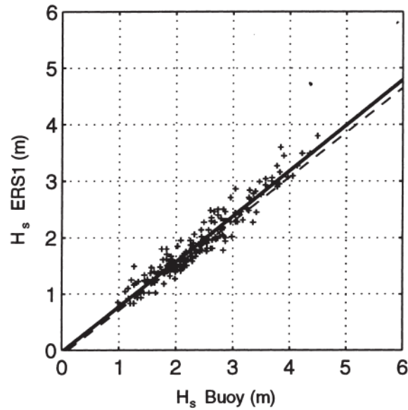
Figure 2.9: Mean monthly values of buoy H_s , compared with mean month values of ERS1 altimeter H_s . The solid line is Equation (2.3-3), and the dashed is the relationship proposed by Cotton and Carter [13] [37]
