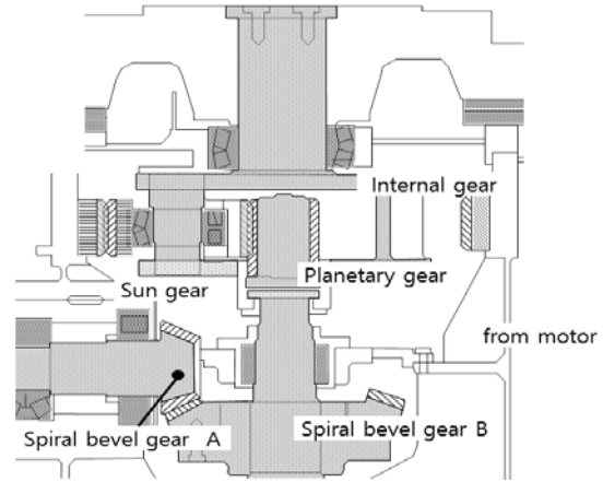
Figure 1. Detailed image of gearbox components.
