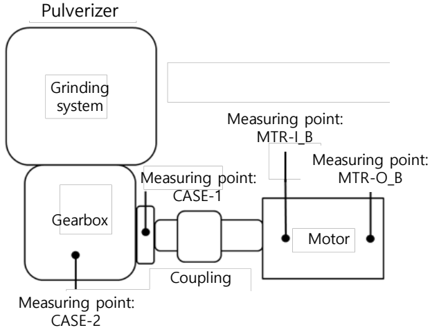
Figure 2. Power transmission of pulverizers: from an electric motor through a gearbox to a grinding system.
