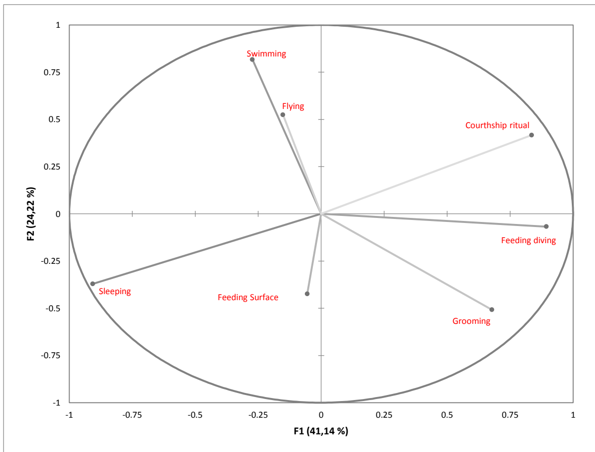
Figure 5: PCA map of the diurnal time budget activities of the White-headed Duck at Garaet Hadj Tahar (Guerbes Sanhadja eco complex). F1 axis eigenvalue= 2.88, variability= 41.14%.
