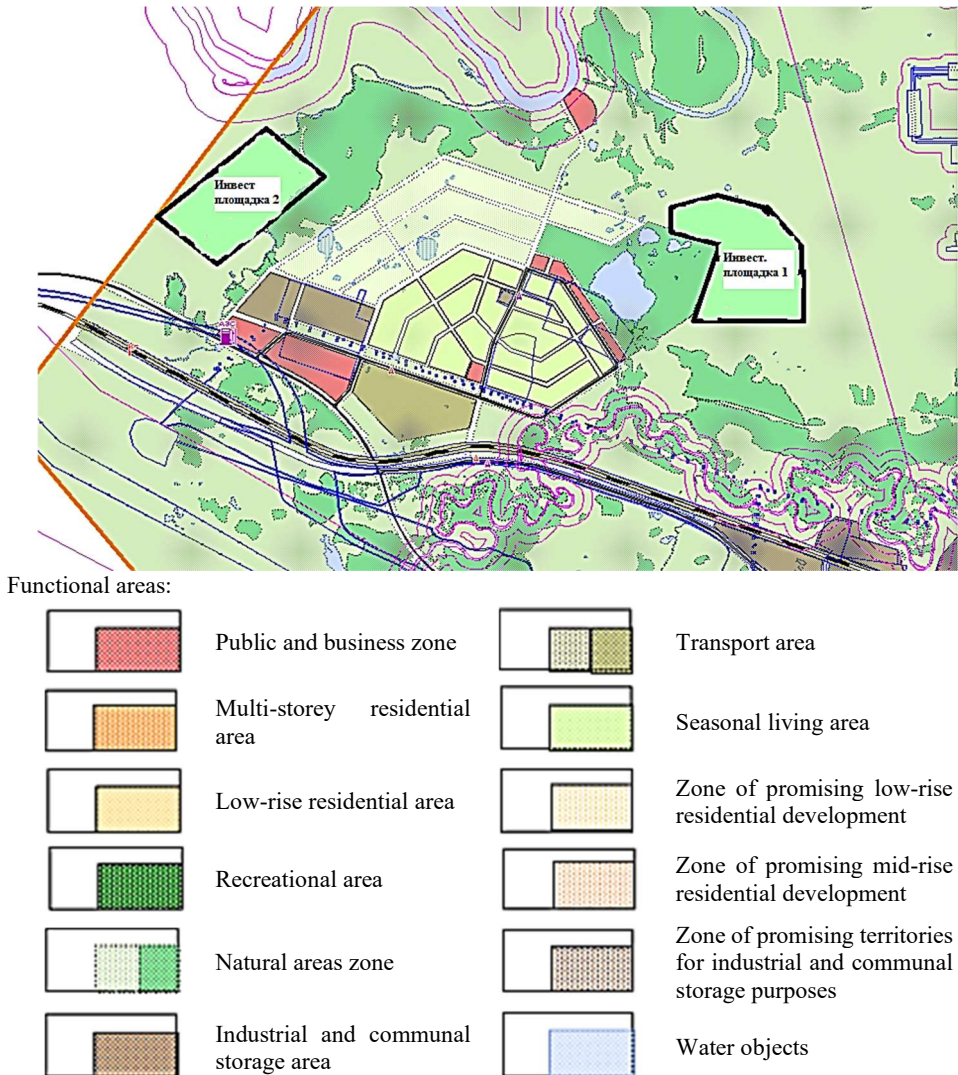
Fig. 1. The preliminary zone of the wind farm facility on the territory of the urban district of the city of Novy Urengoy according to the master plan.
