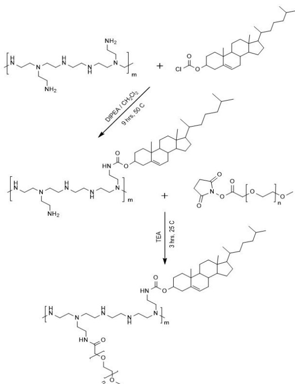
Scheme 1. Schematic presentation of the synthesis of PEI-cholesterol and the consecutive PEGylation reaction.
