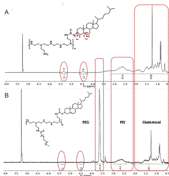
Fig. 2. ^1\text{H-NMR} spectrum of F3 (A) and F5 (B) lipopolymers at the respective mole ratios of 1:15.5:0 and 1:15.5:2 (PEI/cholesterol/PEG) in \text{CDCl}_3 .
