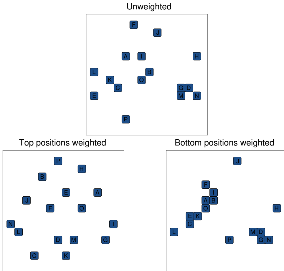
Figure 2 ■ MDS visualization based on the unweighted, top-position weighted, and bottom-positions weighted Kendall distances between people’s preferences for the months of the year. Each square/letter indicates a different participant. The distances between the squares/letters represent their similarities according to the Kendall distance.
