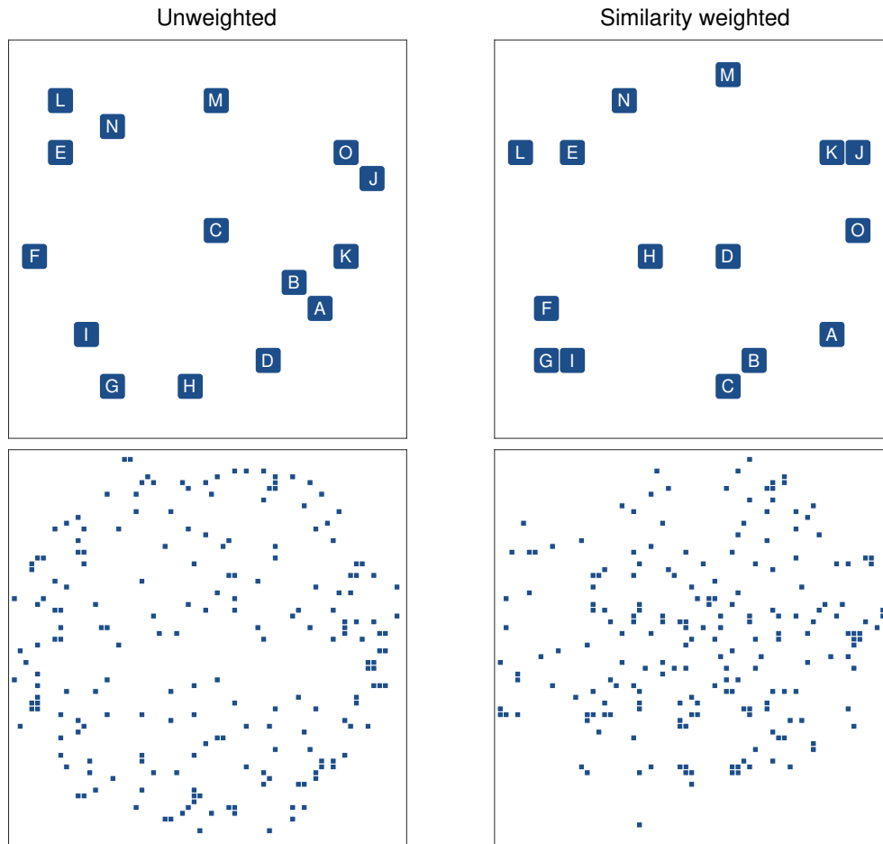
Figure 3 ■ MDS visualization of the similarities between recall patterns of animal names based on the unweighted Kendall distance (left panels) and similarity-weighted Kendall distance (right panels). The top panels show 15 labeled people, while the bottom panels show all 200 people. The distances between the squares/points represent their similarities according to the Kendall distance.
