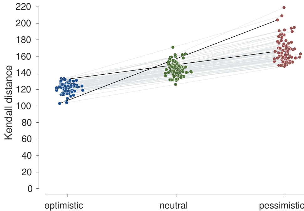
Figure 4 ■ Optimistic, neutral, and pessimistic Kendall distance measures of accuracy for 85 experts from fantasypros.com . Each expert predicted the fantasy football performance of kickers in week 10 of the American National Football League 2017 season. Each point corresponds to a participant, jittered around the Kendall distance measure. The same participant for each measure is connected by a gray line. Experts A and B from Table 3 are highlighted by black lines.
