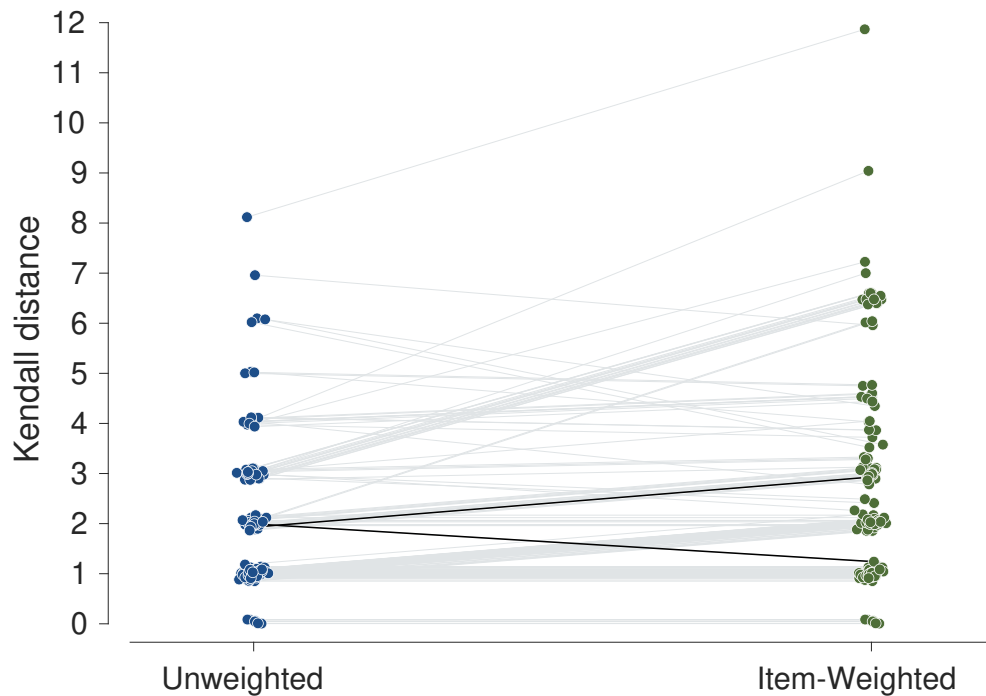
Figure 1 ■ Unweighted and item-weighted Kendall distance for 158 participants from the Altmann (2003) study of memory for the order of events on September 11. The distances are between the participants’ responses and the ground truth. Each point in the unweighted column and item-weighted column corresponds to a participant, jittered around the Kendall distance measure. The same participant for each measure is connected by a gray line. Participants A and B are highlighted by black lines. As a result of the weighting, Participant A sees a decrease of the Kendall distance, whereas Participant B sees an increase of the Kendall distance.
