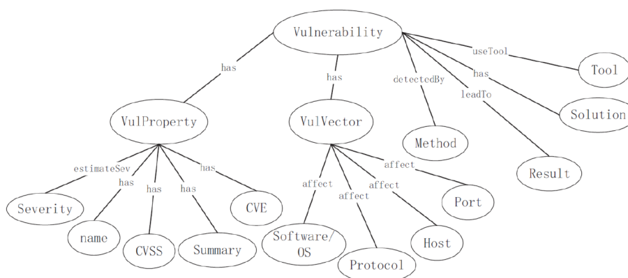
Figure 2: Vulnerability ontology structure
