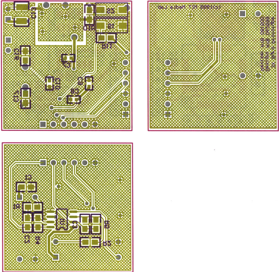
Figure C-3: Main IMU PCB - Bottom
