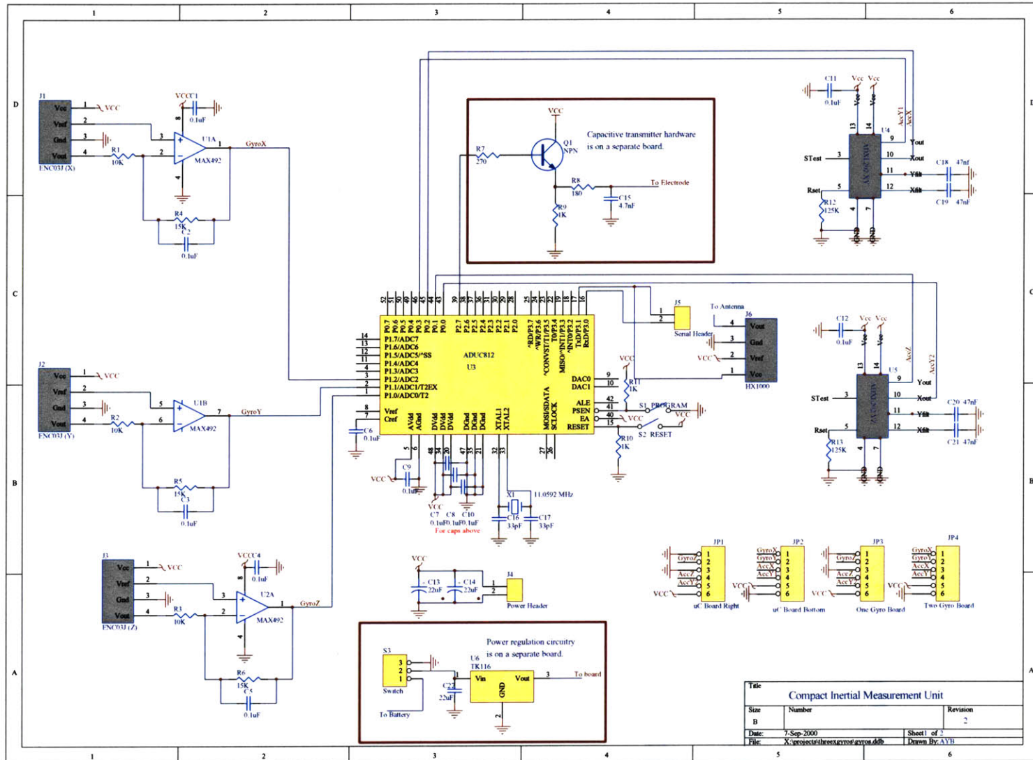
Figure C-1: Main IMU Schematic
