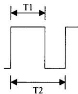
Figure 2-4: ADXL202 Digital Output
