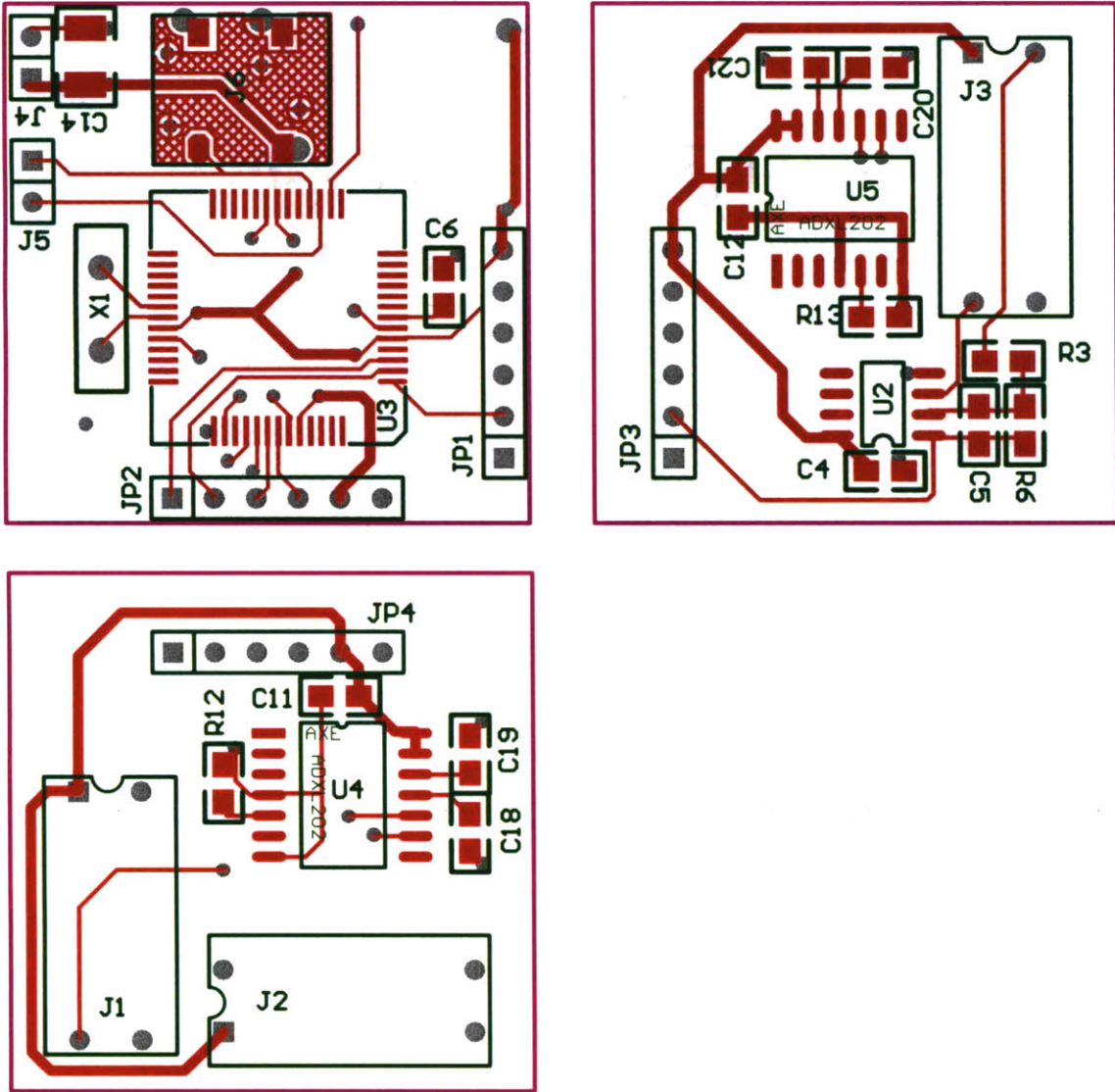
Figure C-2: Main IMU PCB - Top
