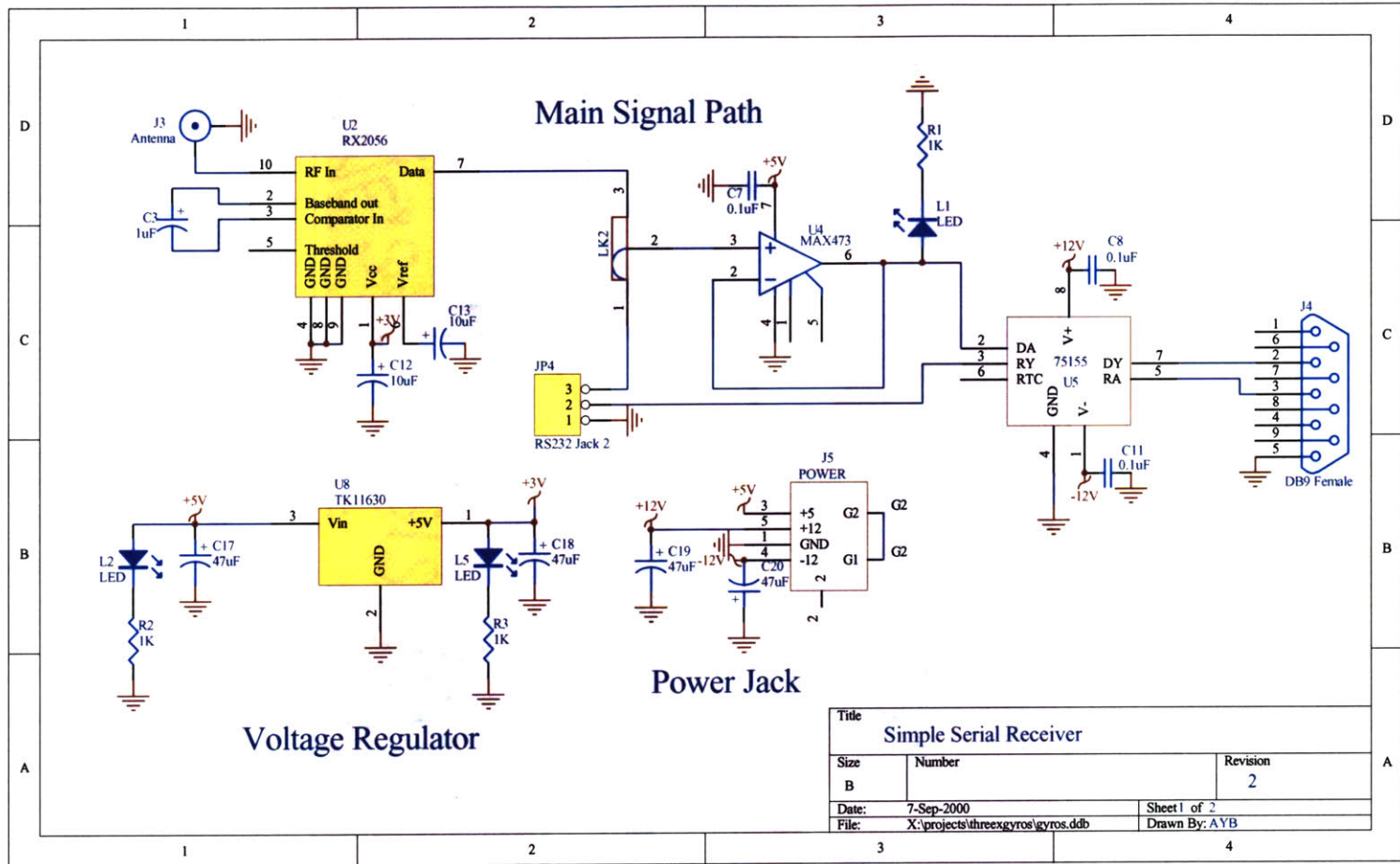
Figure C-4: Receiver Schematic
