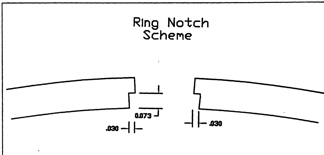
Figure 3-2: Ring End-gap Notching Scheme
