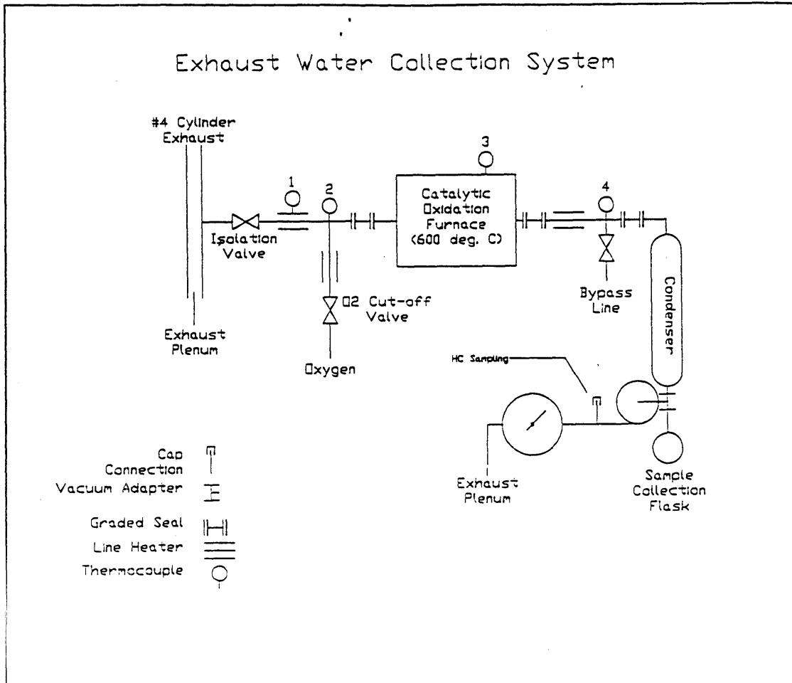
Figure 3-5: WCS Schematic
