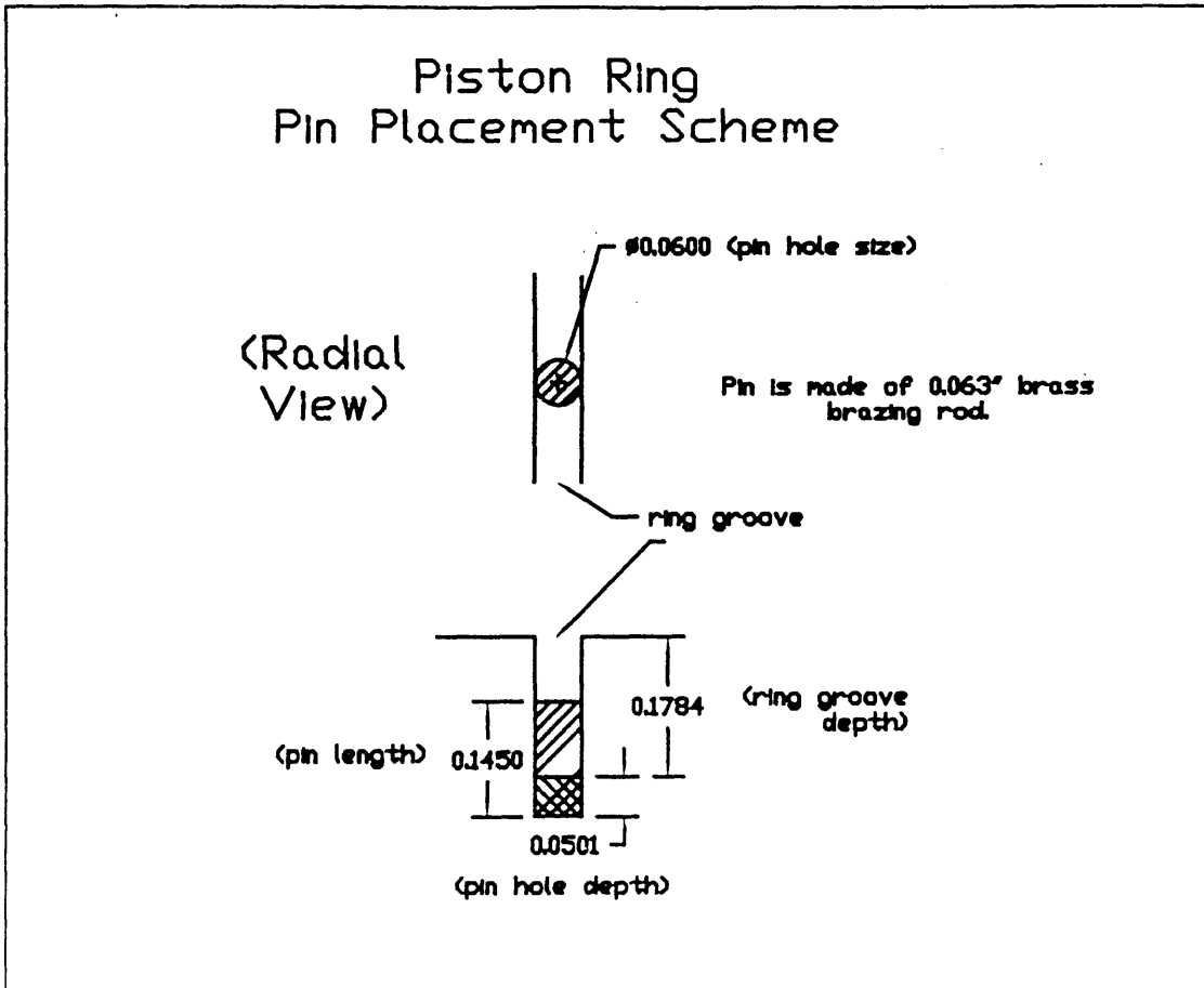
Figure 3-1: Pin Schematic
