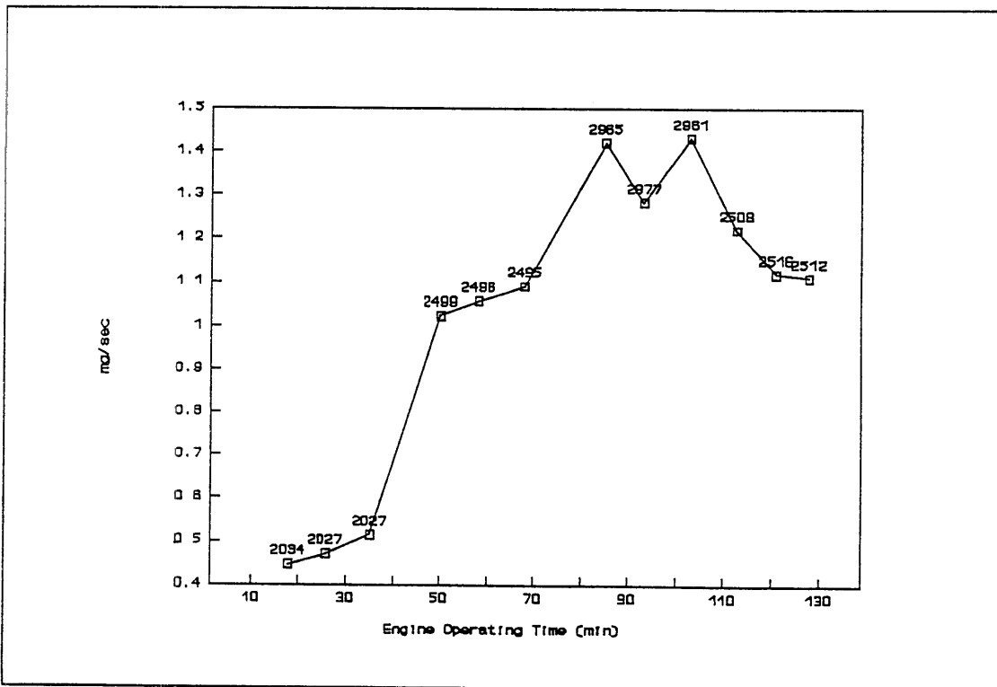
Figure 5-7: OC vs. Time: AZ5
