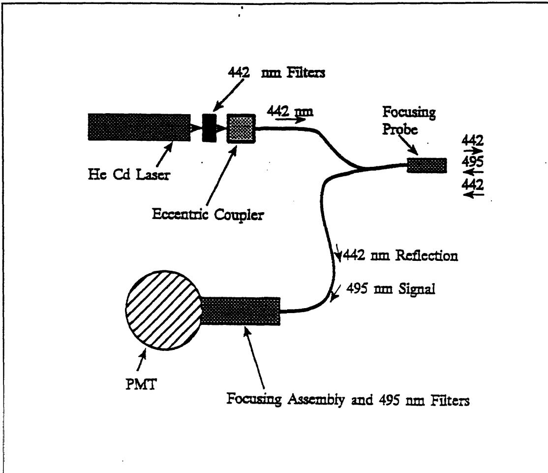
Figure 2-7: LIF Schematic
