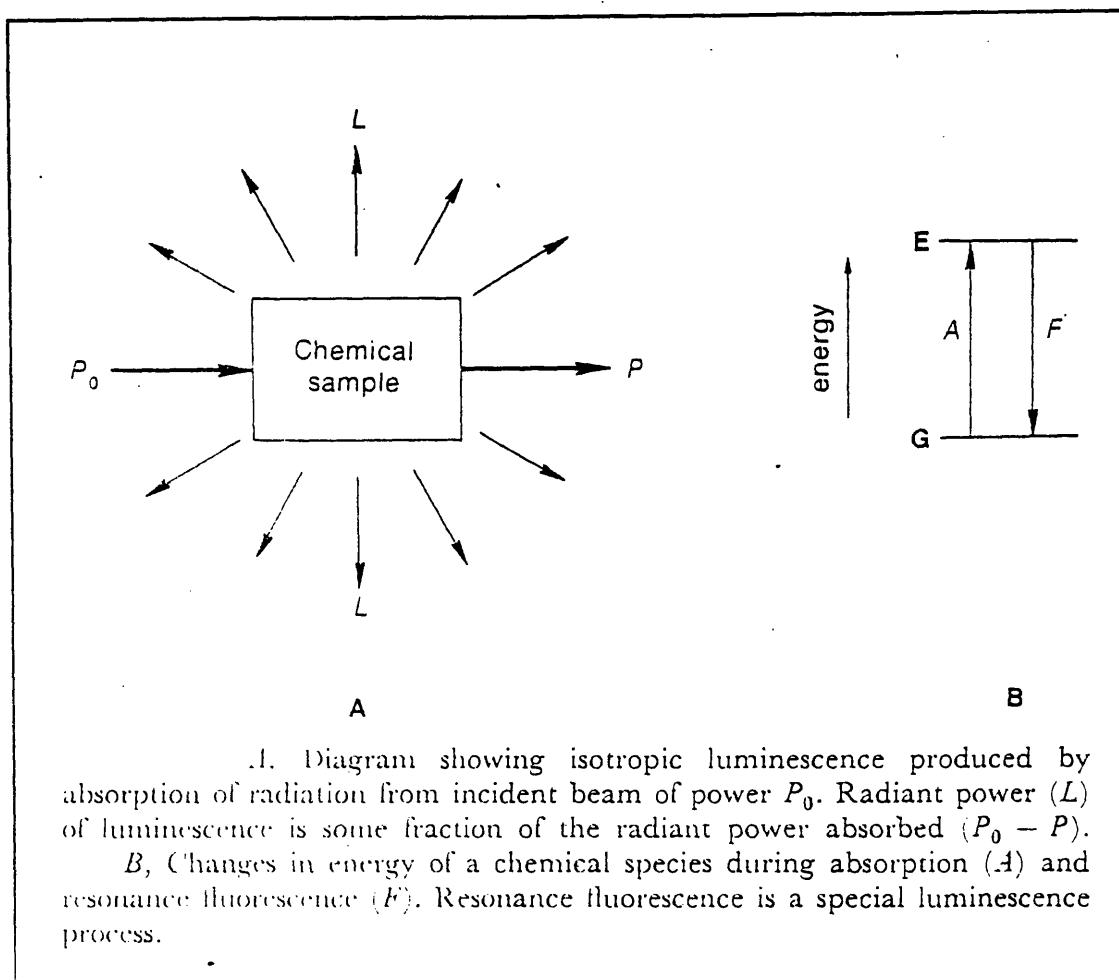
Figure 2-5: Luminescence Process
