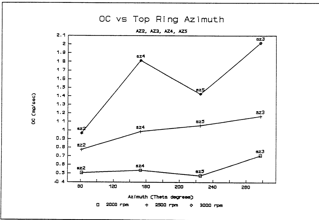
Figure 5-9: Average OC vs. Azimuth
