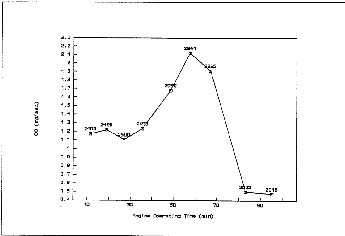
Figure 5-5: OC vs. Time: AZ3
