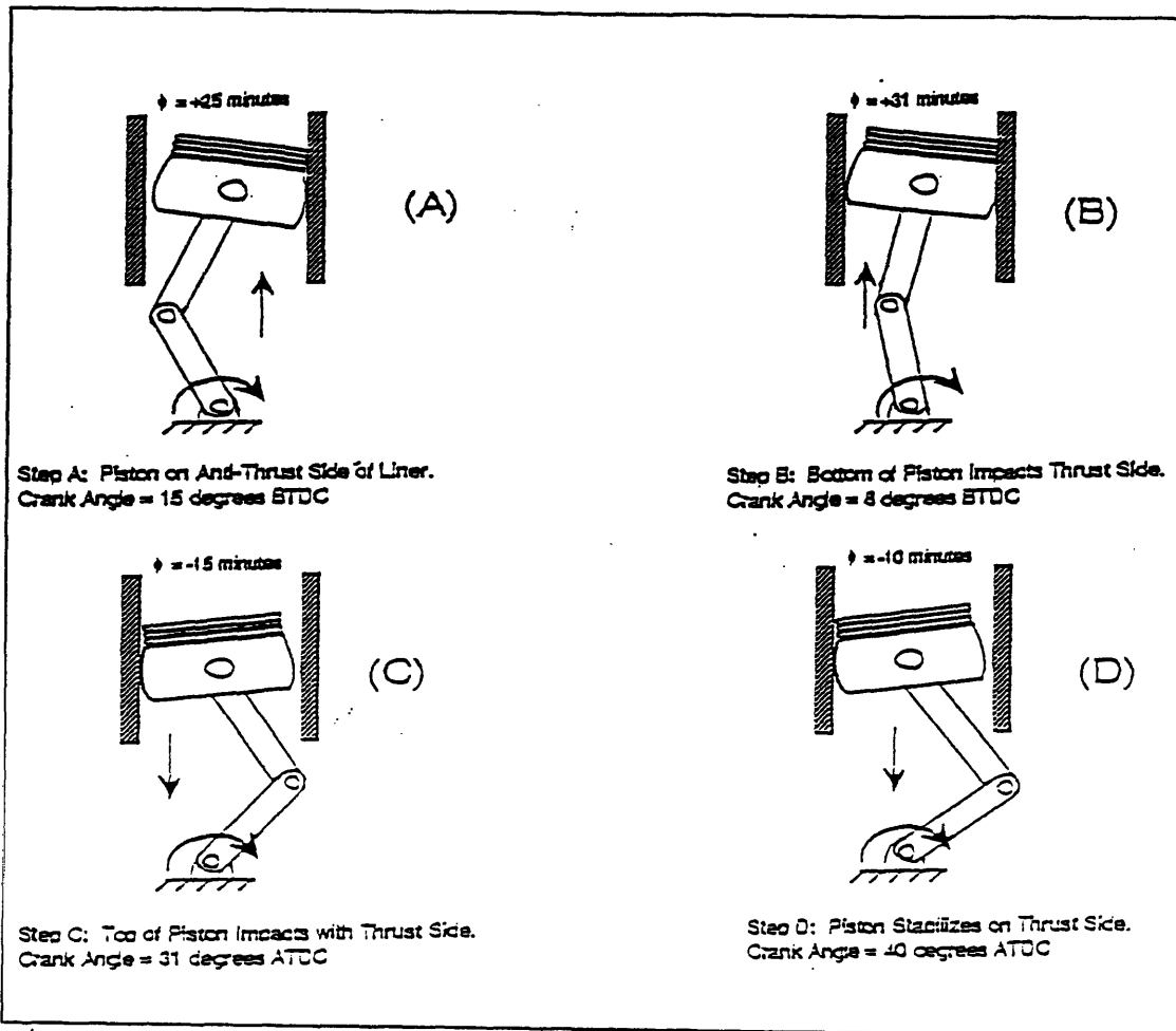
Figure 5-21: Conceptual Sequence of Piston Slap
