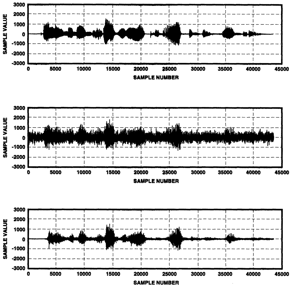
Figure 2-3: Top to bottom : Clean speech waveform representing the utterance “Aluminum silverware can often be flimsy”; speech waveform corrupted by white noise at an SNR of 0 dB; enhanced waveform produced by the sequential/adaptive algorithm.
