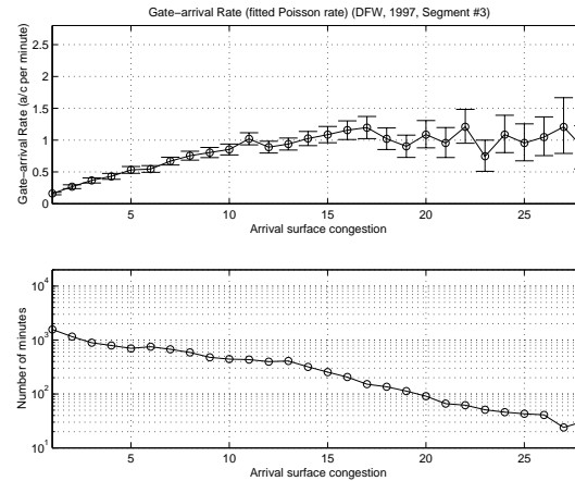
Figure 21: Gate throughput at DFW (inclement weather).
