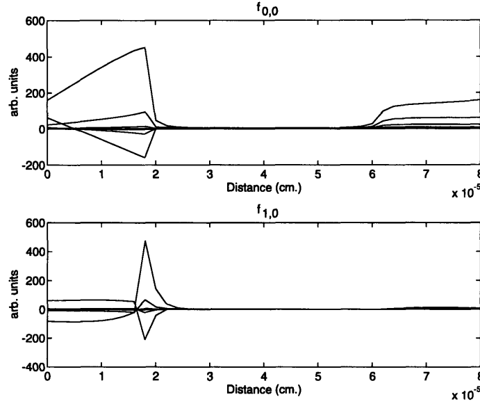
Figure 3-10: Unstable results obtained using the one-sided scheme.
