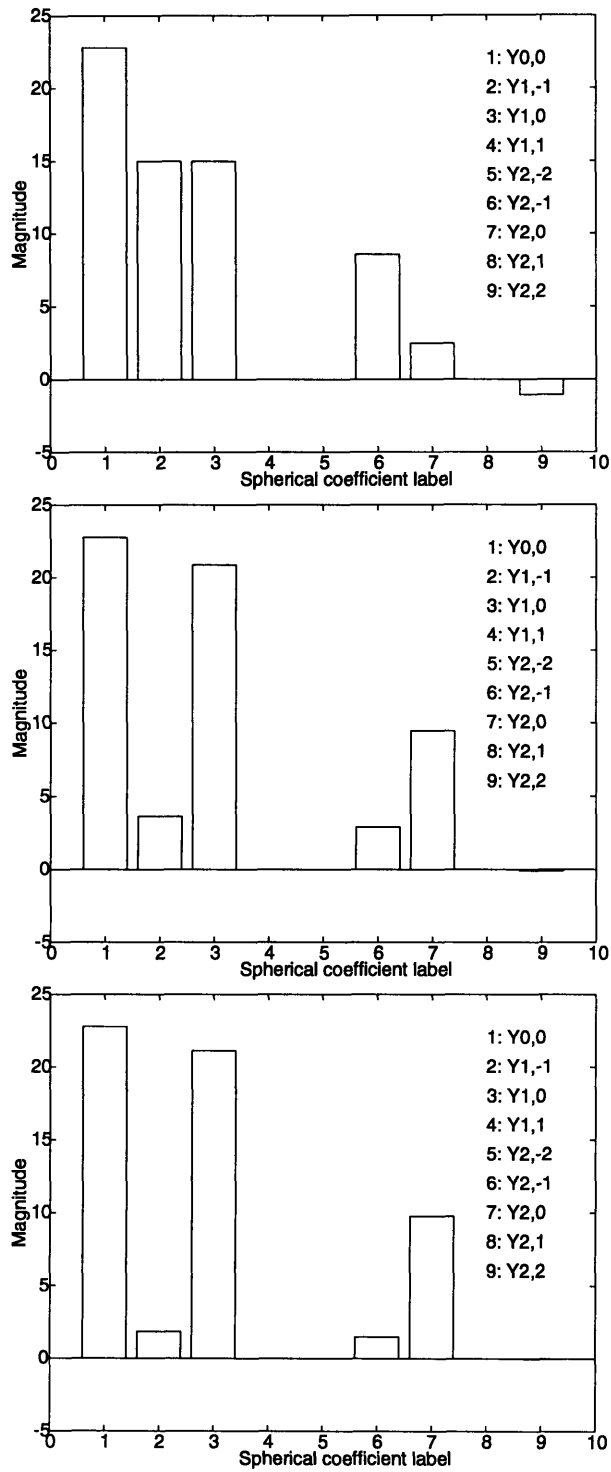
Figure 4-3: Coefficients of the spherical harmonics up to second order for a Maxwellian distribution displaced from the origin along directions 45°, 10°, and 5° from the origin.
