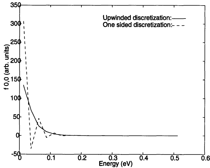
Figure 3-12: A comparison of the solution for f_{0,0} obtained using the one-sided (dash) and upwinded (solid) discretization schemes.
