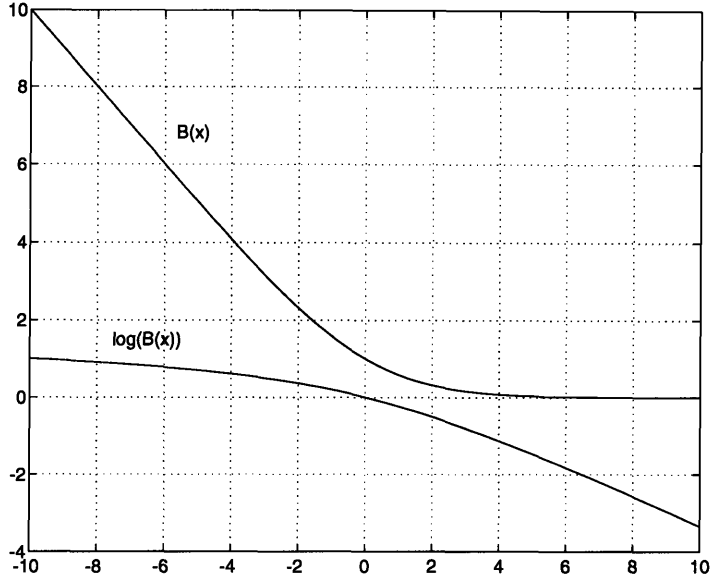
Figure 2-3: Bernoulli function and its logarithm
