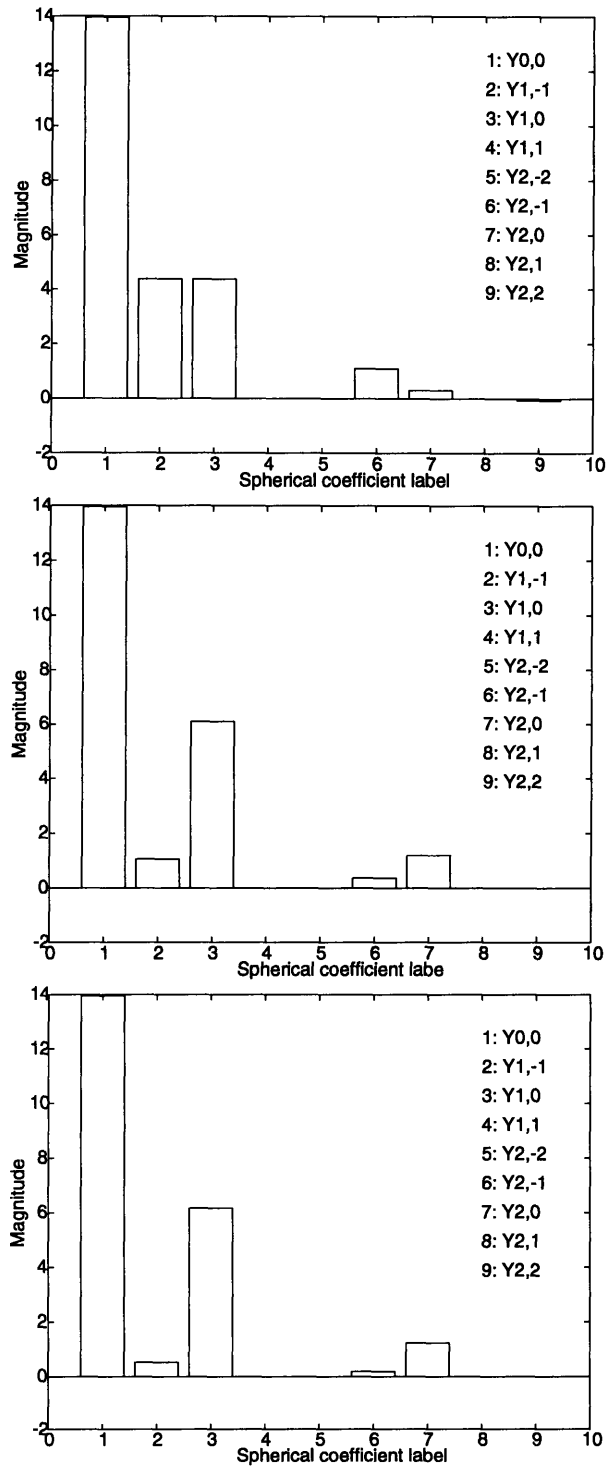
Figure 4-2: Coefficients of the spherical harmonics up to second order for a Maxwellian distribution displaced from the origin along directions 45^\circ , 10^\circ , and 5^\circ from the origin.
