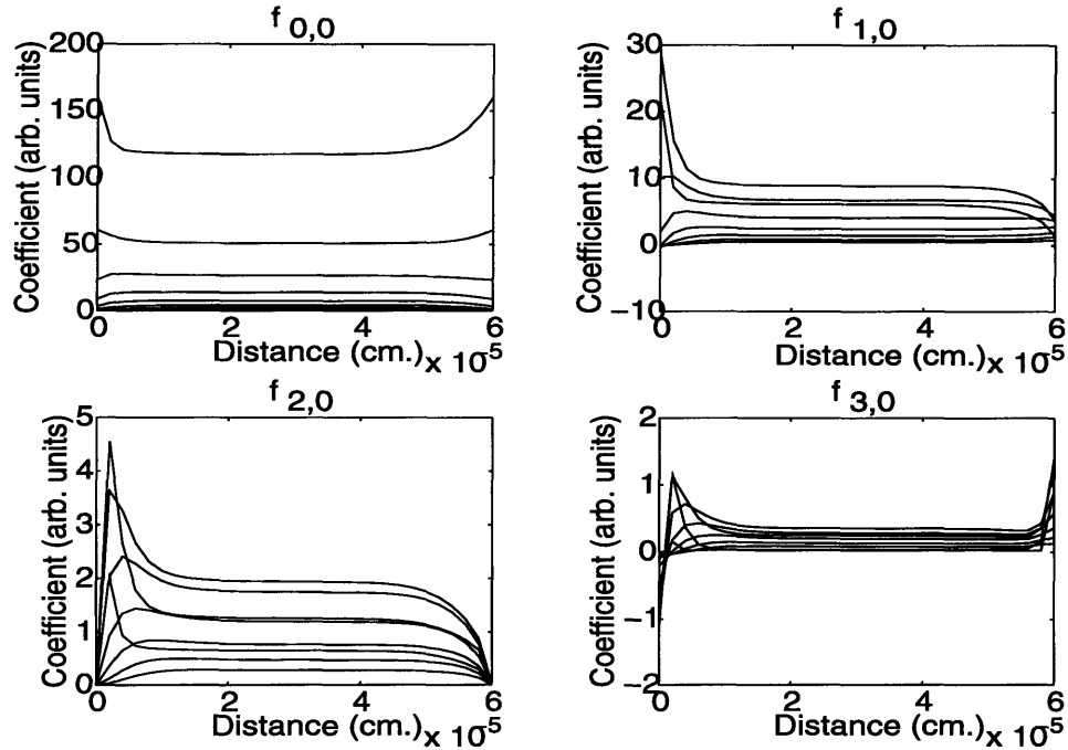
Figure 3-15: Zero to third order coefficients as a function of position for different electron energies (25meV spacing in energy) for the 0.6 μm resistor shown in the previous figure.
