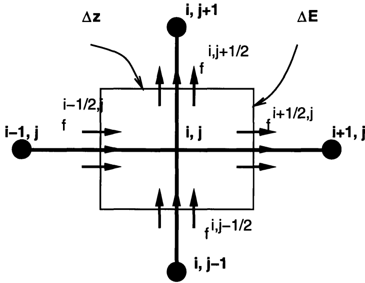
Figure 3-7: Control volume for energy-space discretization.
