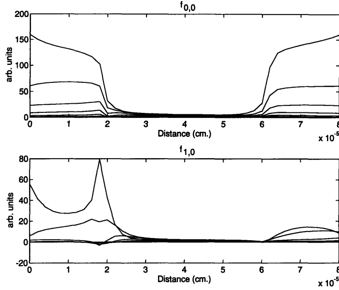
Figure 3-11: Stable results obtained using the upwinded scheme.
