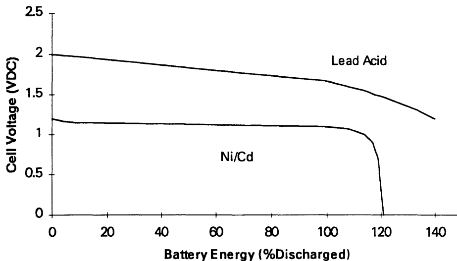
Nickel-Cadmium Discharge Characteristic (with Lead Acid Superimposed) [25, 63]
