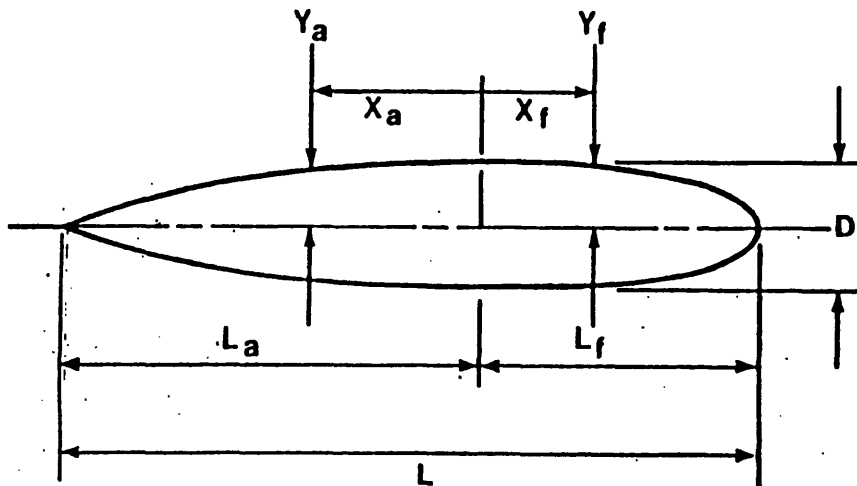
The Body of Revolution Hull
