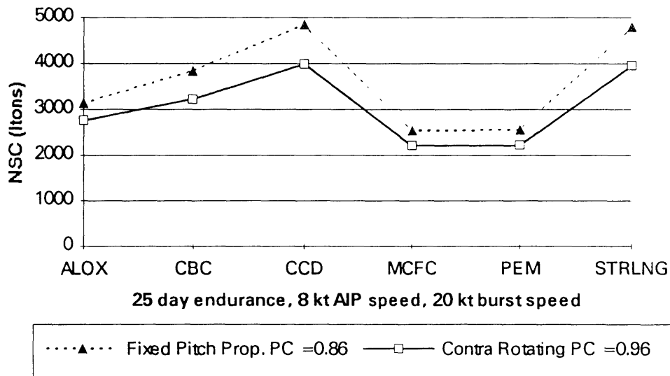
Effect of Propulsive Coefficient on NSC
