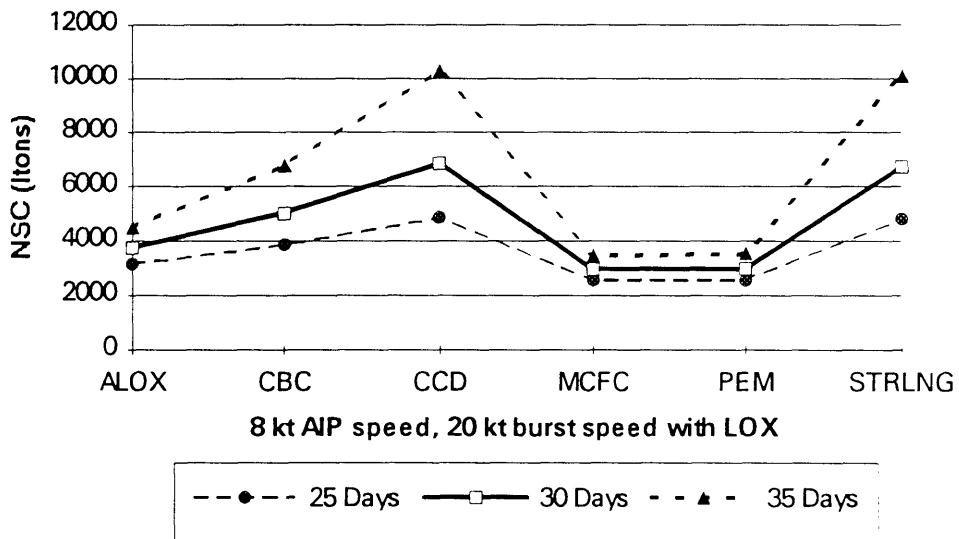
AIP Plant Variation with Endurance
