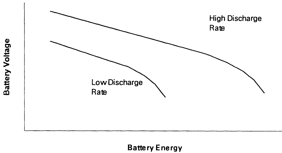
Typical Lead Acid Discharge Characteristic [41]
