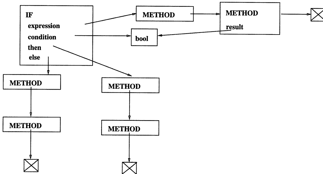
Figure 6-4: If Node
