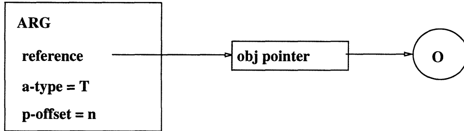
Figure 6-1: Var Arg Node
