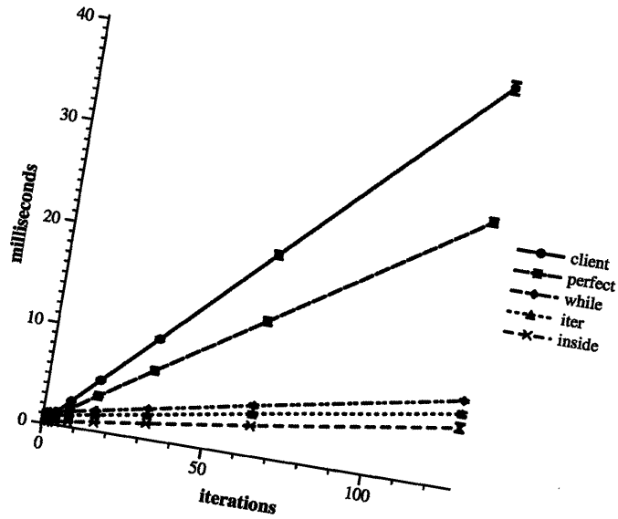
Figure 7-1: BCS Performance
