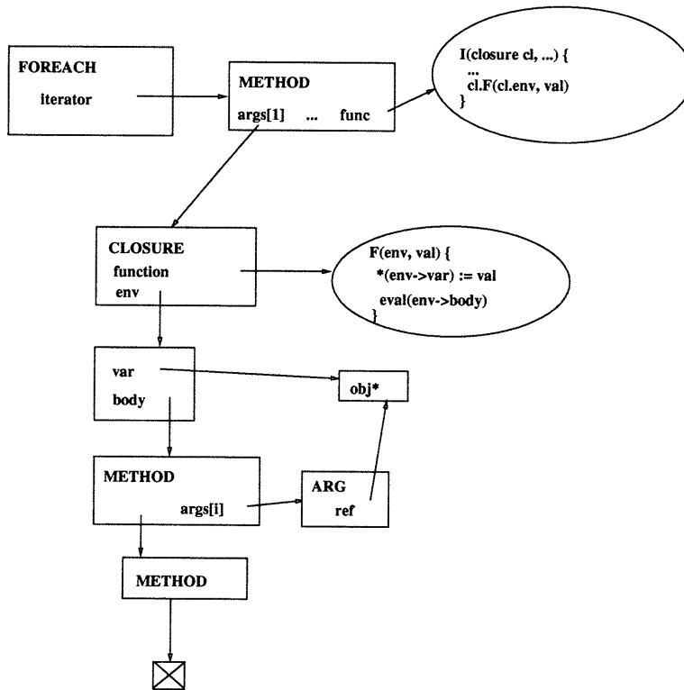
Figure 6-6: Foreach Node
