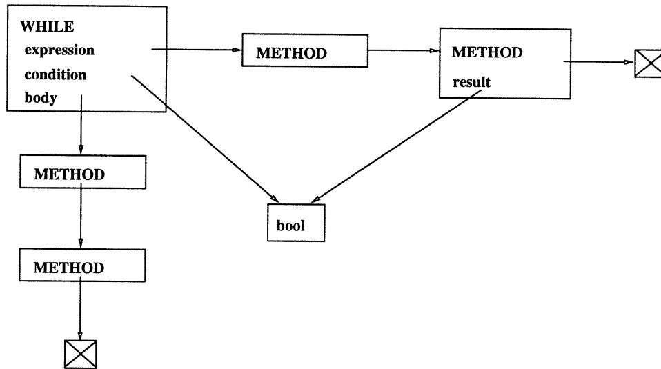
Figure 6-3: While Node
