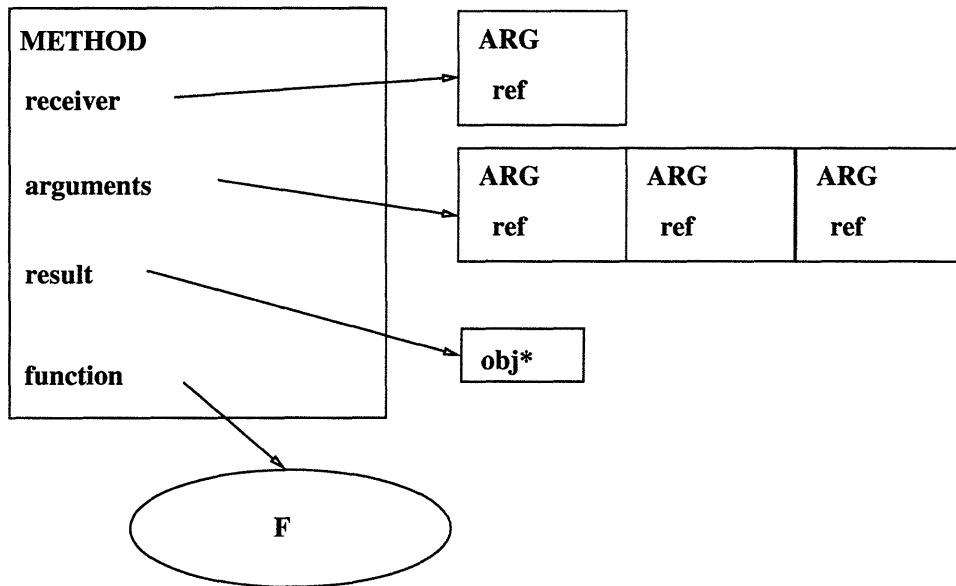
Figure 6-2: Method Node
