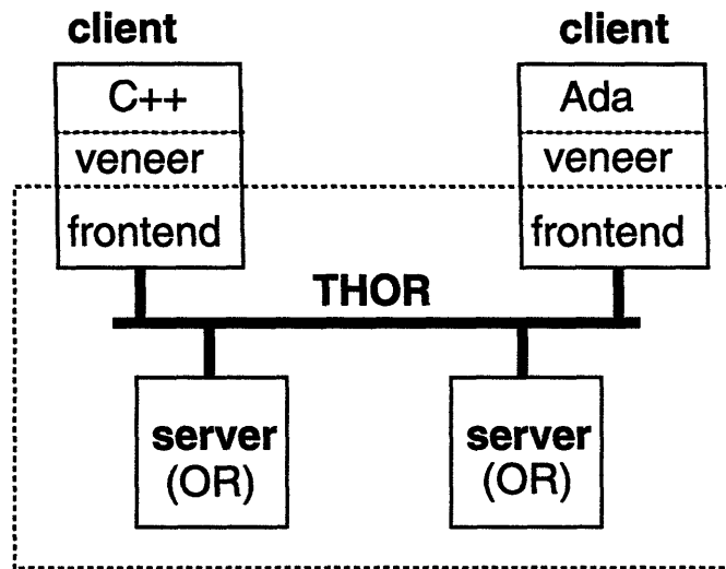
Figure 2-1: Thor architecture.
