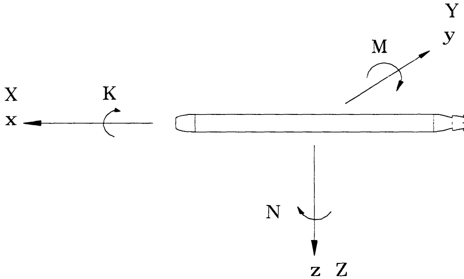
Figure 2.3 Body-Fixed Axis, Force and Moment Conventions for a UUV
