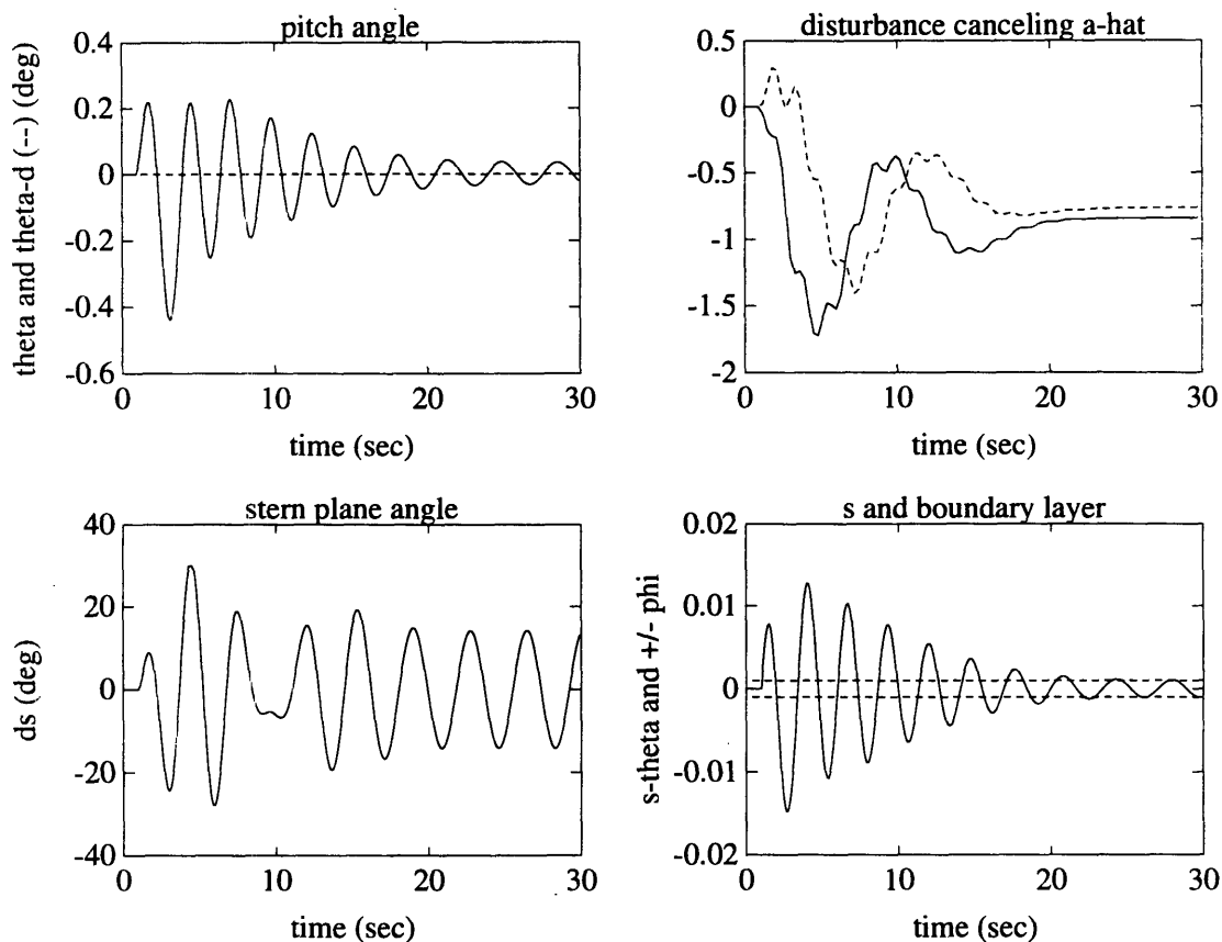
Figure 5.18 Adaptation to a Single Frequency Disturbance by the Pitch Controller. Here, \Gamma = \text{diag}[\Gamma_\theta, 100\mathbf{I}] . Performance is improved with this controller which uses two disturbance cancellation terms, \hat{a}_7 \sin(1.7t) and \hat{a}_8 \cos(1.7t) , to adapt to and cancel the pitch disturbance of known frequency, but of unknown phase and magnitude. Pitch response is significantly reduced from the previous cases, with final control action magnitude comparable to that of the previous two controllers. The error parameter, s_\theta is seen to decrease in amplitude so that it becomes bounded by \Phi_\theta , which implies that s_{\theta\Delta} \rightarrow 0 .
