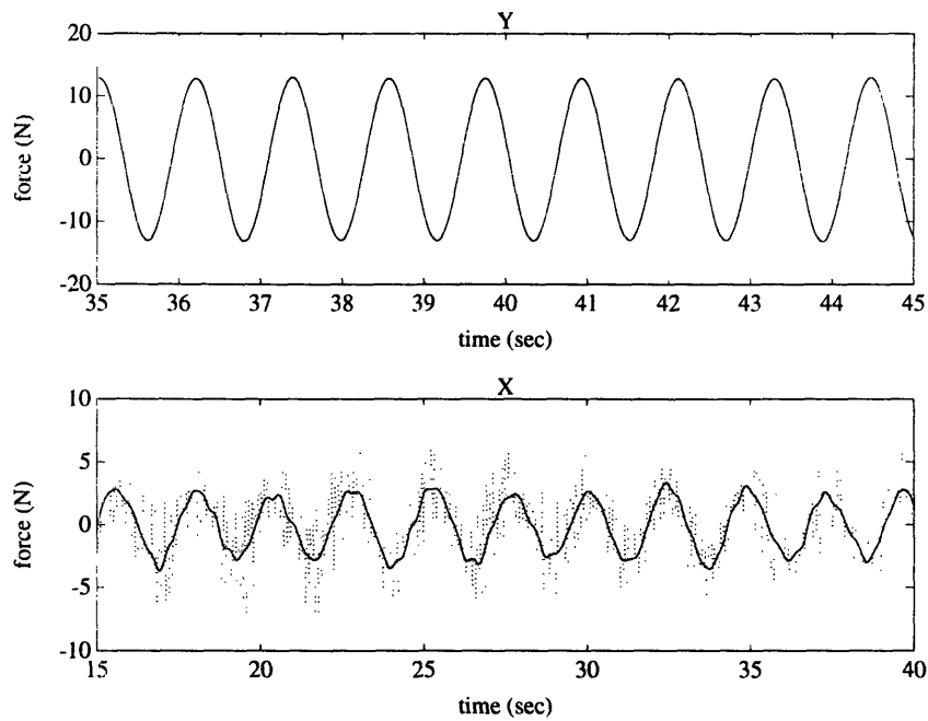
Figure 3.5 Two Samples of Unfiltered and Filtered Signals
