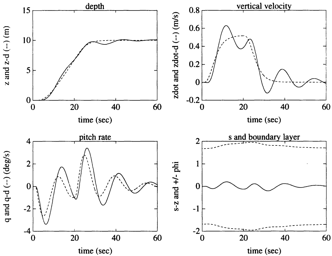
Figure 5.6 21UUV Depth Trajectory with Adaptive Sliding Pitch Control Law, \Gamma = 0 . Here, the pitch control law from equation (5.33) is used with no adaptation of parameter estimates. This pitch controller is very similar to the robust sliding controller used previously, differing only in that the feedback gain k_{\theta_{eff}}(t) from the robust sliding controller is approximated by a constant, k_{\theta} = 7 . Speed and depth controllers remain unchanged. As expected, depth trajectory following is very similar to that depicted in figure 5.2.
