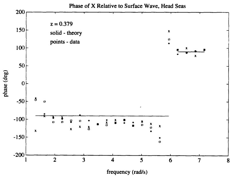
Figure 3.6b Surge Force Transfer Function Phase for Shallow Model in Head Seas
