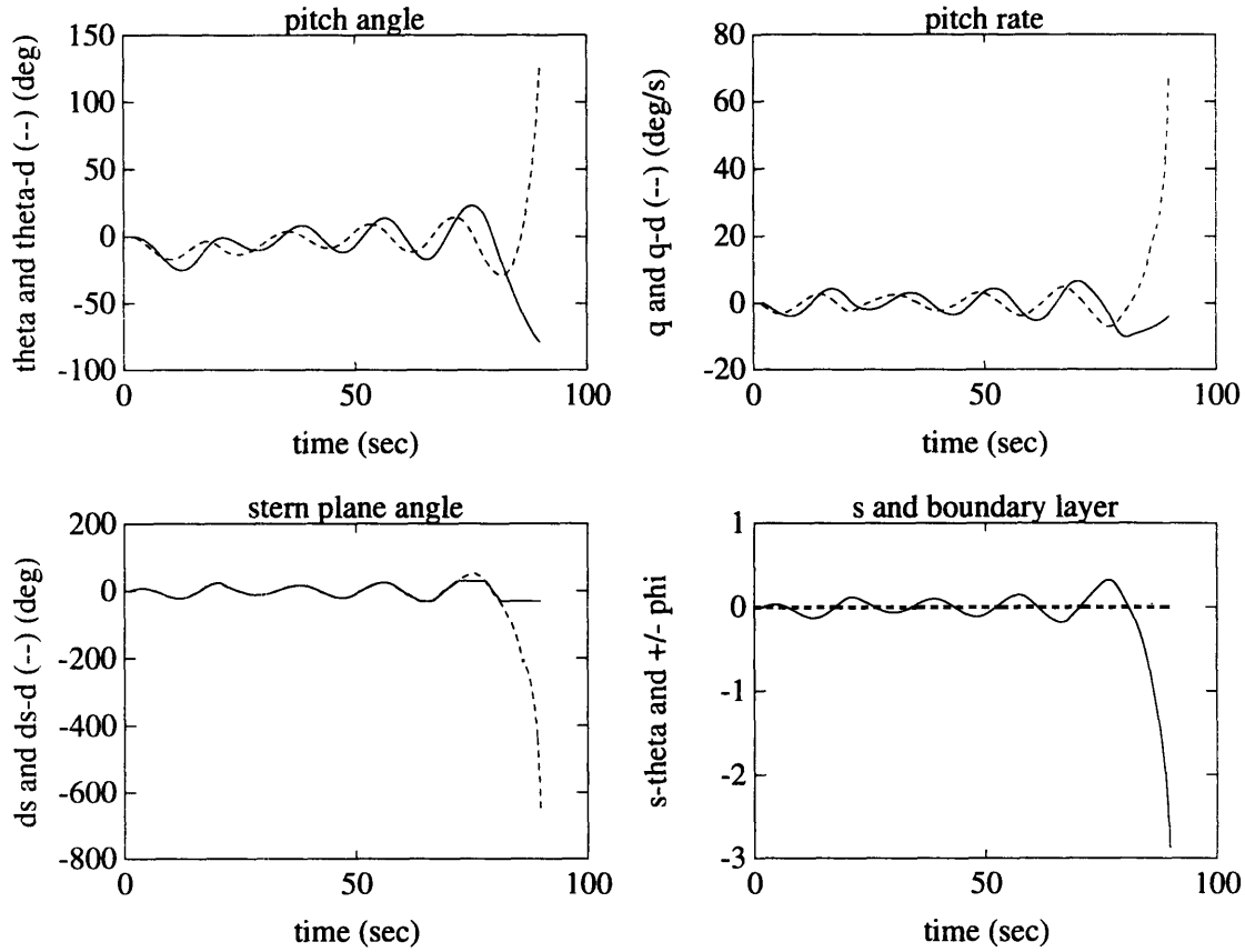
Figure 5.12 21UUUV Pitch Response with Adaptive Sliding Pitch Control Law, \Gamma = \mathbf{0} . The pitch control law from equation (5.33) is used, and controller constants remain k_\theta = 7 and \Phi_\theta = 0.012 . \hat{\mathbf{a}} = \hat{\mathbf{a}}(0) is derived using an assumption of no prior knowledge of hydrodynamic constants except for M_{\delta_1} , which is known to within 30% error as before. The estimates of body coefficients remain unchanged. Parametric uncertainty and the lack of parametric adaptation leads to instability of this pitch controller.
