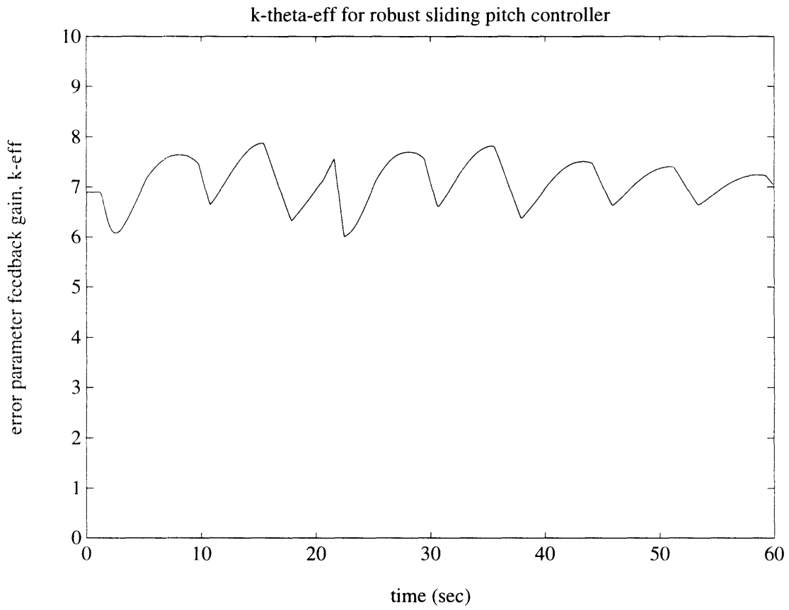
Figure 5.5 Robust Sliding Pitch Controller k_{\theta\text{eff}}(t) . Though k_{\theta\text{eff}} varies with time, it is seen that k_{\theta\text{eff}} \approx 7 for the duration of this depth change maneuver.
