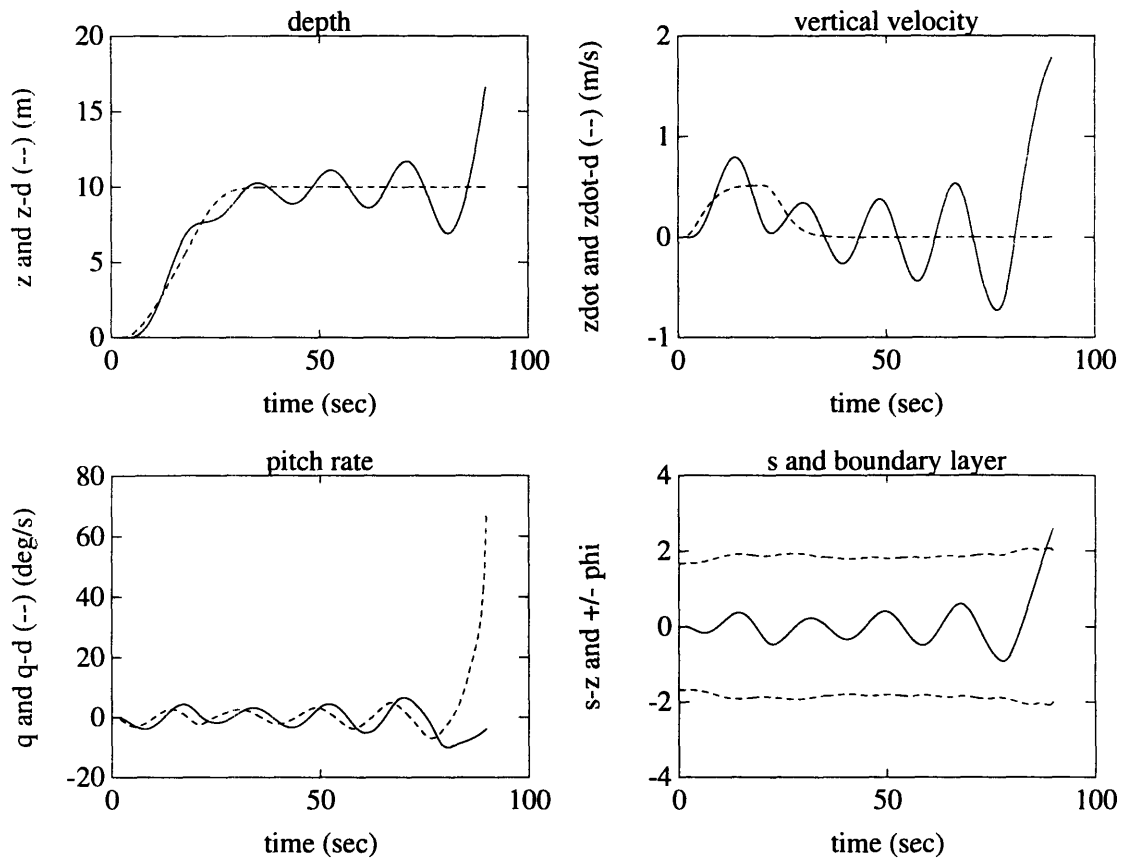
Figure 5.11 21UUV Depth Trajectory with Adaptive Sliding Pitch Control Law, \Gamma = \mathbf{0} . Here, the pitch control law from equation (5.33) is used with no adaptation of parameter estimates, and the depth and speed controllers remain unchanged. In this case, it is assumed that there is no prior knowledge of the hydrodynamic coefficients except for M_{\delta_s} , which is known to within 30% error as before. Body coefficients, as before, are assumed known to within 5% error. Because parametric uncertainty is so high, without adaptation this control scheme is unstable.
