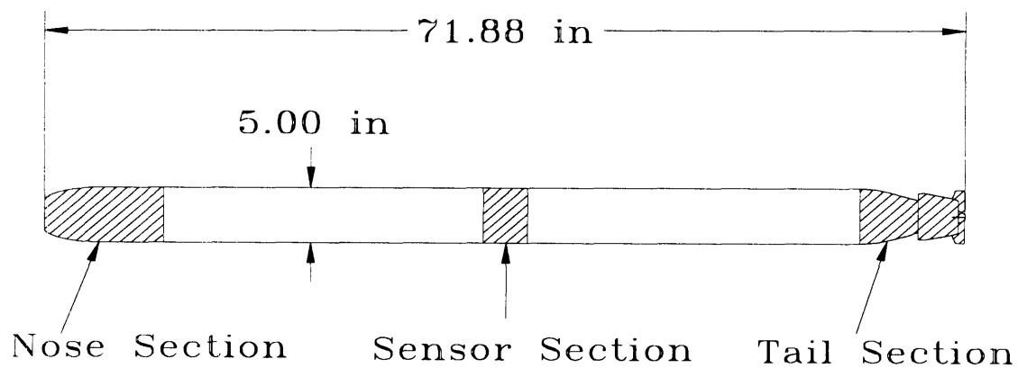
Figure 3.2 21UUV Model Used in Testing
