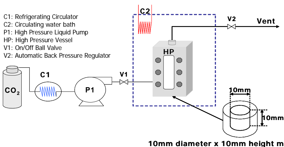
FIGURE 1. Experimental Setup for supercritical gas foaming technique
