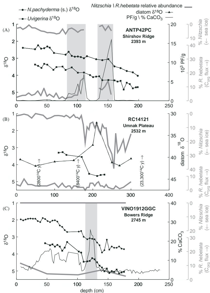
Fig. 4. Shaded bars represent “green” layers, which are characterized by high \% \text{CaCO}_3 , \% C_{\text{org}} , and \% \text{opal} . \delta^{18}\text{O} data is of Uvigerina with hispid test in (A), (B), and (C). The thin line in (C) is \% \text{CaCO}_3 , in (A) it is # planktonic foraminifera (PF) per gram dry sediment, a proxy for \% \text{CaCO}_3 . Presence of Nitzschia is associated with sea ice, R. hebetata is associated with high nutrient availability and C_{\text{org}} flux. Nitzschia abundance patterns show that maximum extent of sea ice may not have reached the Bowers or Shirshov Ridge core sites during the LGM or YD. Note that the x-axis scales are not the same between the panels. The y-axis scales for a property on each panel are identical. Previously reported in Sancetta et al. (1985) were the diatom \delta^{18}\text{O} data and the three uncorrected, uncalibrated ^{14}\text{C} dates in (B), which were measured on the organic fraction of 20 cm-thick sections of sediment and interpreted as maximum, not exact ages, establishing the uppermost lithologic unit of this core (0–175 cm) as Holocene.
