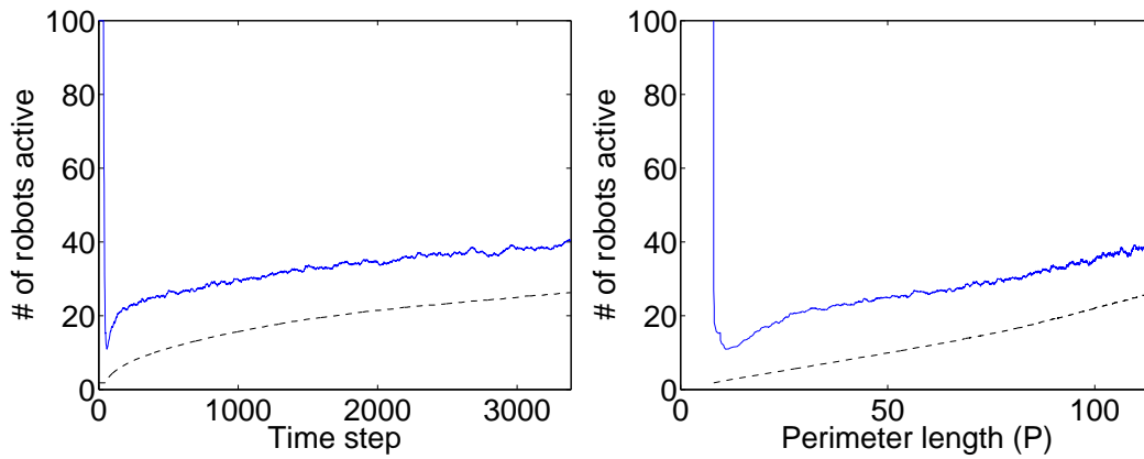
Figure 4-12: Number of active robots as a function of time (left) and of perimeter length (right), with adaptive recruiting as described in the text. The dotted line shows P/(A + 1) \cdot (1 + L/(A + D)) . L = 31 , A = 11 .
