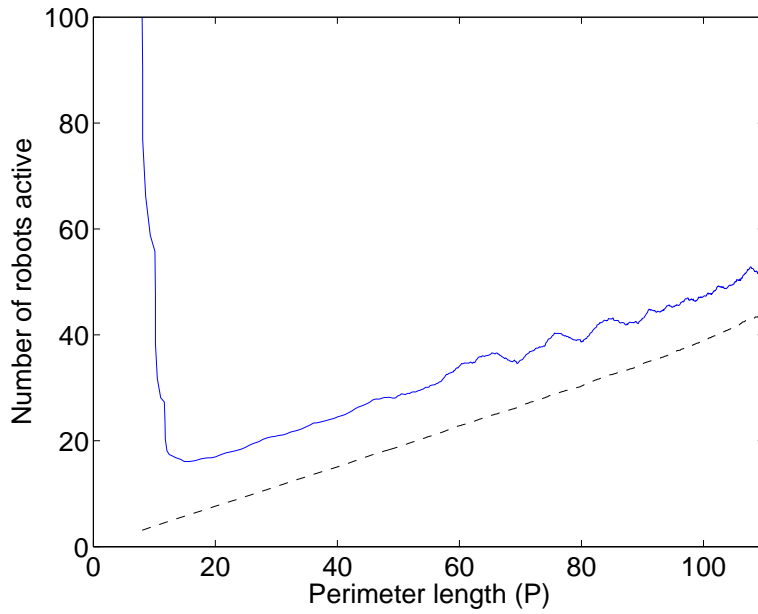
Figure 4-11: Number of active robots as a function of length of the structure perimeter, with adaptive recruiting as described in the text. The dotted line shows P/(A + 1) \cdot (1 + L/(A + D)) . L = 1 , A = 1 .
