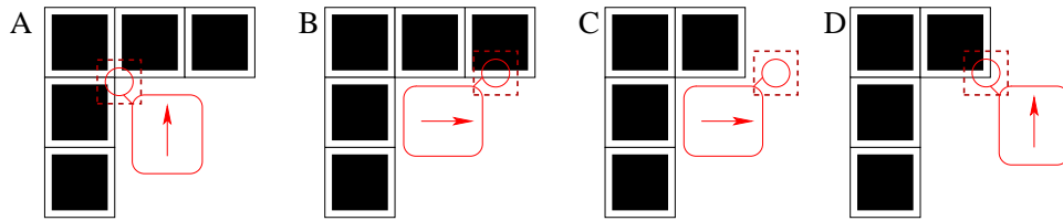
Figure 5-4: When the robot turns right at an inside corner, it may not be able to back up far enough at the end of the turn for the camera to see the structure. (A) Before the turn. (B) After the turn, if the wall now to the robot’s left continues far enough, the camera can see it and wall-following can continue. (C) If the wall is not visible, the robot infers a left-turn corner and performs a modified left-turn sequence to put it at the position shown in (D).
