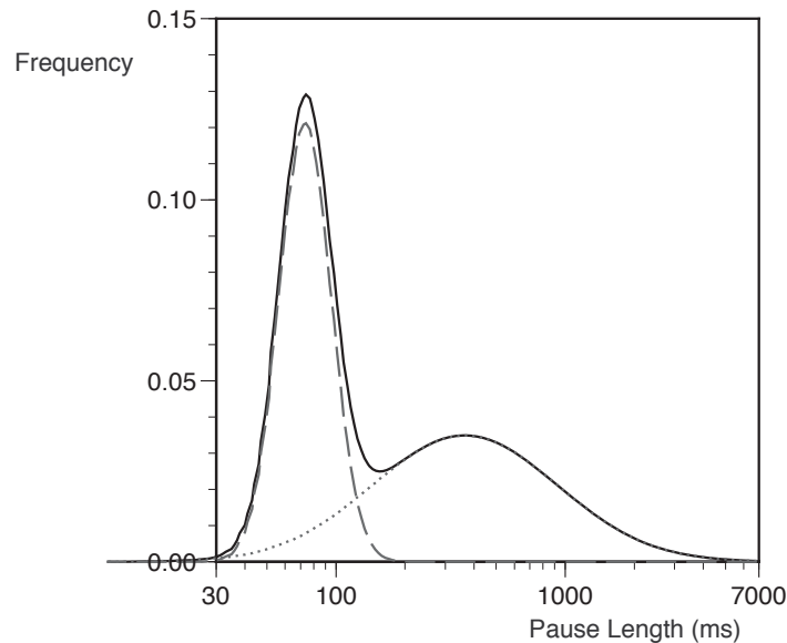
Figure 5-23: This figure shows the Gaussian estimations for each class and the sum of the two estimates for speaker 1. The dashed line is the Gaussian estimate for the within-phrasal class of pauses. The dotted line is the Gaussian estimate for the between-phrasal class. The solid line is the sum of the two Gaussian estimations.
