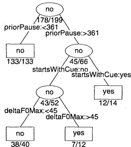
Figure C-1: CART tree for classifying SBEG phrases for speaker 4.
