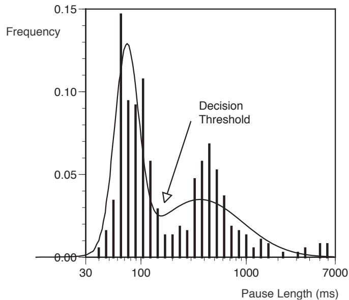
Figure 5-24: This figure shows the sum of the two Gaussian estimations (one for within-phrasal pauses and one for between-phrasal pauses) overlaid on the raw pause histogram for speaker 1. The local minimum (155 ms) is selected as the decision threshold. This differs by 6% from the threshold determined using the hand-labeled data (165 ms).
