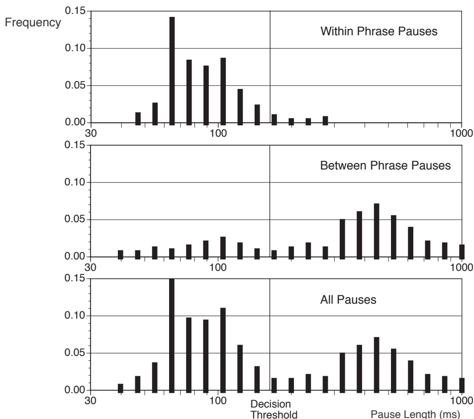
Figure 5-16: Log transformed pause distributions for speaker 1. The bottom plot shows all pauses in the recording. The pauses have been separated into two classes: within-phrase pauses (top plot) and between-phrase pauses (middle plot). For this speaker, the decision threshold that minimizes the number of misclassification errors is at 165 ms.
