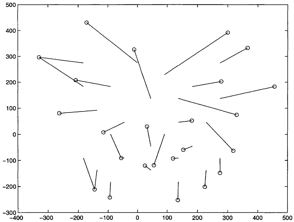
Figure A-1: Initialization results for the 27 node 2D experimental topology. Initial position estimates are marked with circles. Lines are drawn from these estimates to the corresponding ground truth sensor locations. The average position estimate error is 70 cm.
