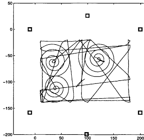
Figure 6-2: Small network setup. Six sensors (squares) are arranged around a rectangular enclosure. A camera captured the ground truth trajectory of the ROOMBA. The ROOMBA followed the trajectory depicted.
