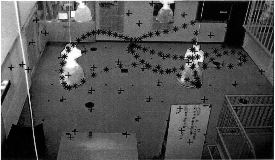
Figure 6-16: Results for the 55 node 3D experiment. Estimated positions are plotted with crosses, and a portion of the recovered mobile trajectory is plotted using asterisks and a dotted line. LaSLAT localized this network with a mean error of 7 centimeters.
