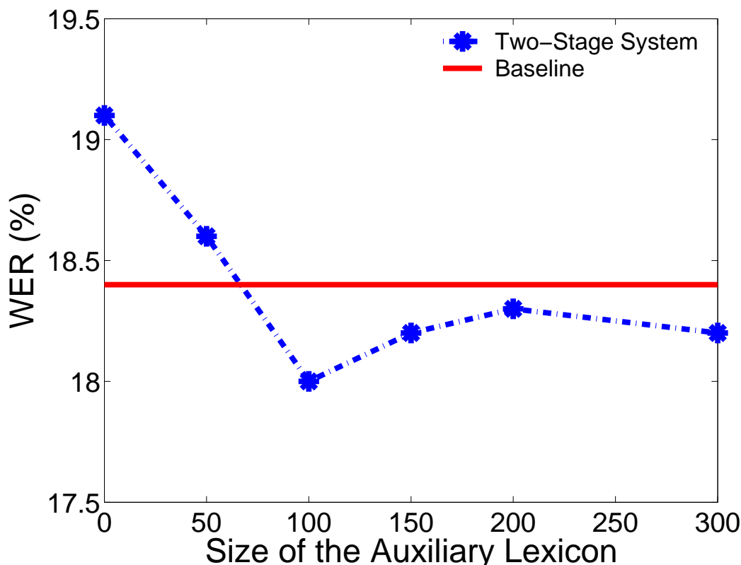
Figure 3-3: Performance dynamics of System II as we increase the number of compensative words.
