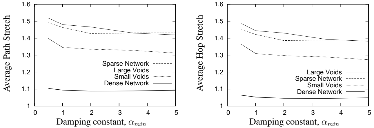
Figure 6-29: Plot of \alpha_{min} against GDSTR stretch.
