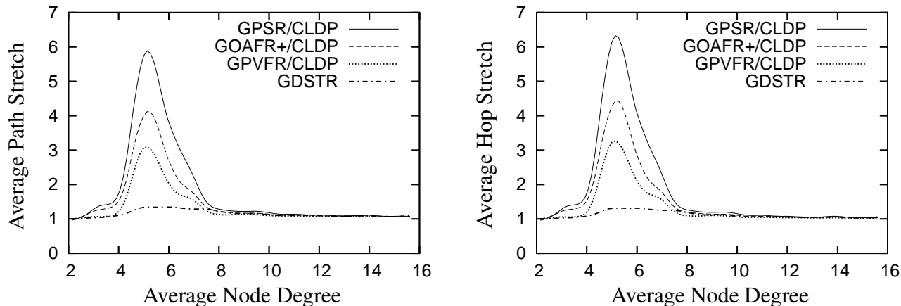
Figure 6-2: Plot of hop stretch with GSpring coordinates.
