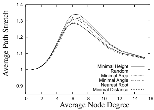
Figure A-12: Effect of the tree choosing heuristic on GDSTR II routing performance.
