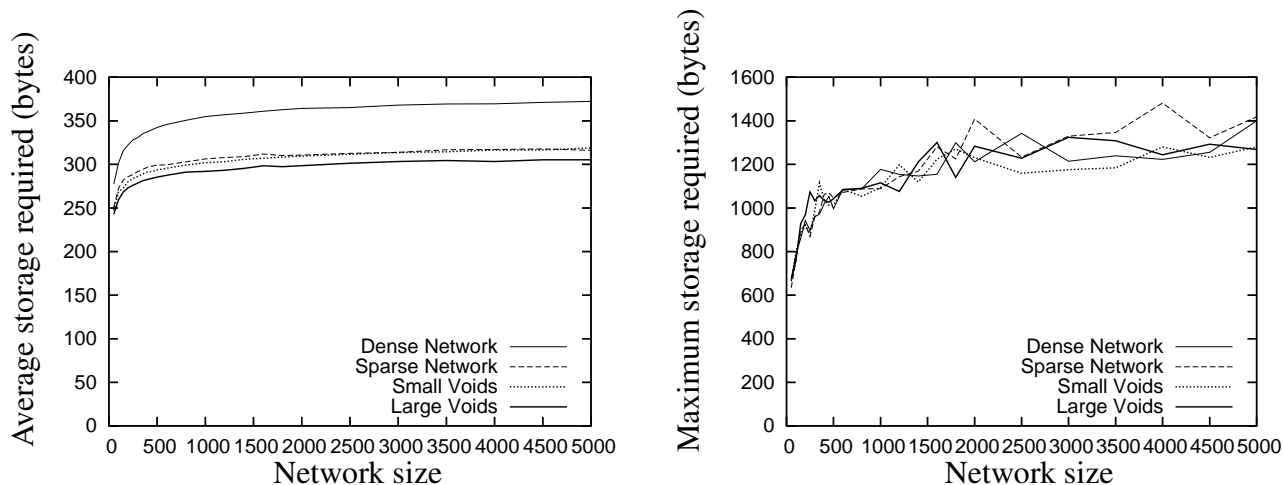
Figure 4-22: Amount of routing state stored at each node for networks with up to 5,000 nodes.
