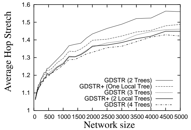
Figure 4-31: Plots comparing the routing performance of GDSTR to GDSTR+ for sparse UDG networks (average node degree 6.5).
