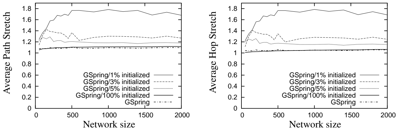
Figure 6-10: Plot of GDSTR stretch with location information seeding for dense UDG networks (average node degree 12).
