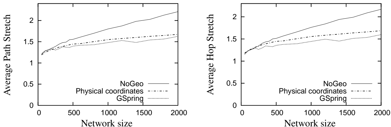
Figure 6-8: Plot of GDSTR stretch for networks with high obstacle density (average node degree 7).
