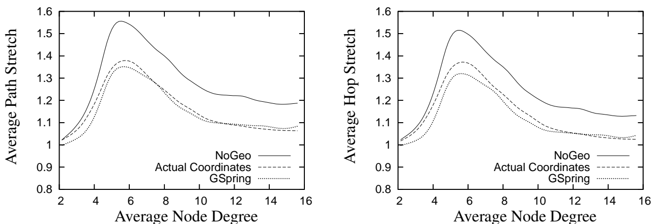
Figure 6-3: Plot comparing the stretch for GDSTR/GSpring over networks of different average node degrees (Note change of scale from Figure 6-2).
