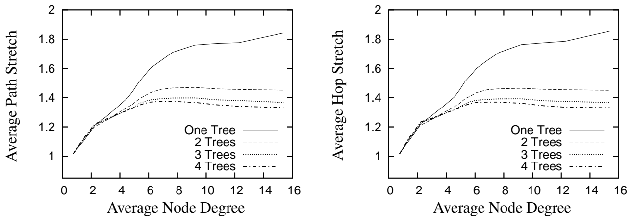
Figure 4-10: Routing stretch performance for GDSTR with different numbers of hull trees for packets that require tree traversal.
