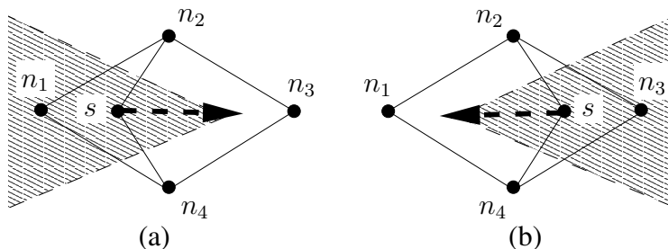
Figure 5-7: Configuration where a node, s , will oscillate and is unable to obtain virtual coordinates that will keep other nodes out of its region of ownership (shaded in gray).
