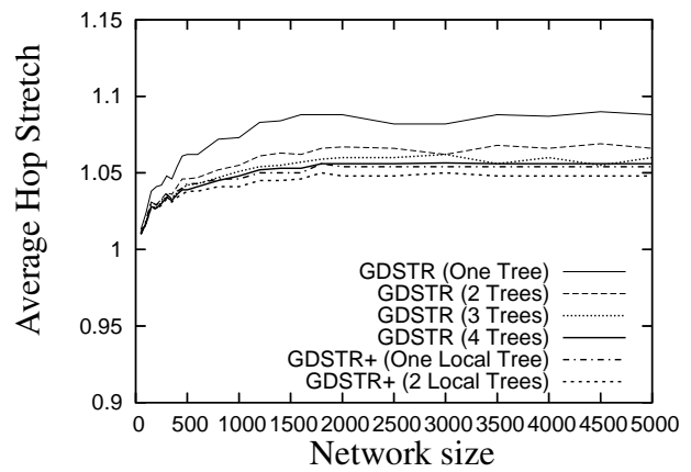
Figure 4-32: Plots comparing the routing performance of GDSTR to GDSTR+ for dense UDG networks (average node degree 12).
