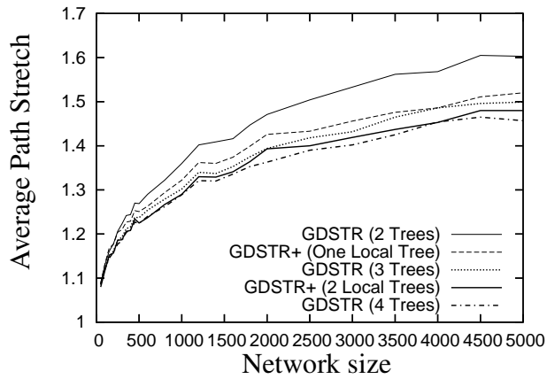
Figure 4-31: Plots comparing the routing performance of GDSTR to GDSTR+ for sparse UDG networks (average node degree 6.5).
