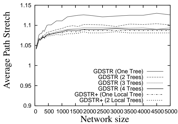
Figure 4-32: Plots comparing the routing performance of GDSTR to GDSTR+ for dense UDG networks (average node degree 12).
