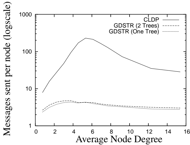
Figure 4-20: Packets sent or forwarded per node when a new node joins (averaged over only the nodes that are affected by a node join or failure).
