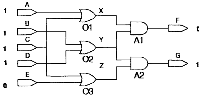
Figure 3-2: An OCSP example, with observed inputs and outputs indicated.
