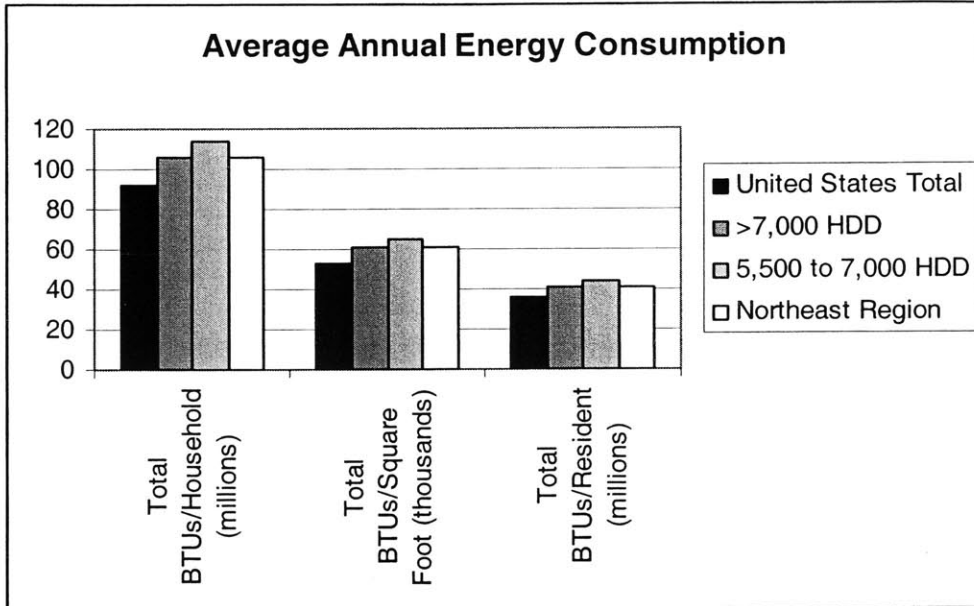
Figure 3.3: Average Annual Energy Consumption
