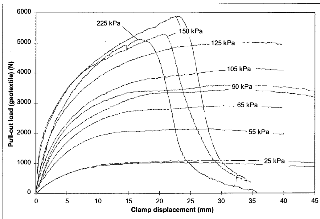
Figure 6-13: Effect of confining pressure on the pull-out load versus clamp displacement relationship
