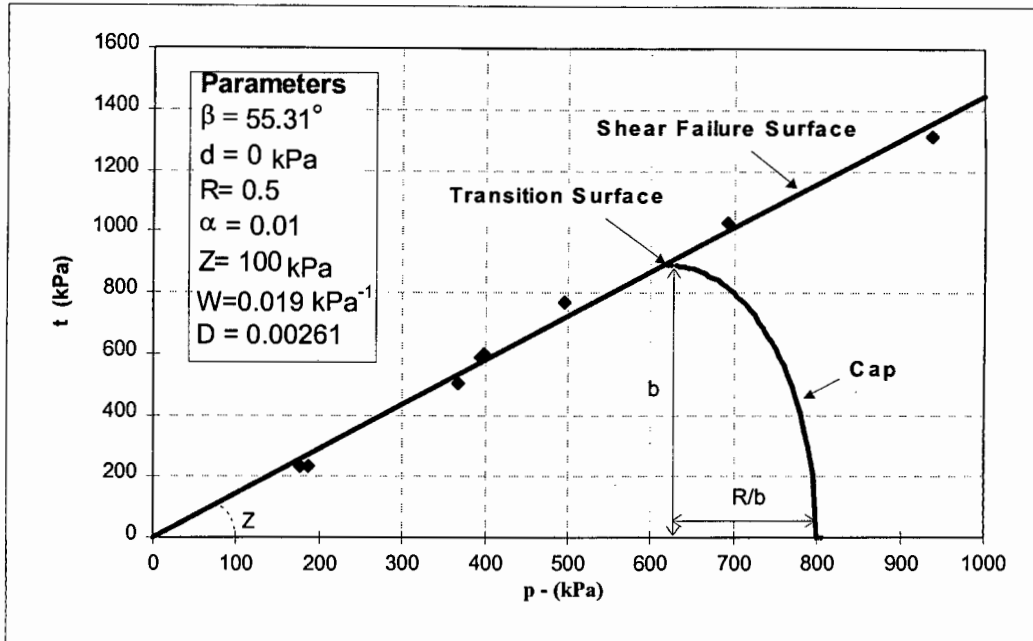
Figure 8-8: Drucker-Prager Cap plasticity model implemented in the finite element program to model Cape Flats sand
