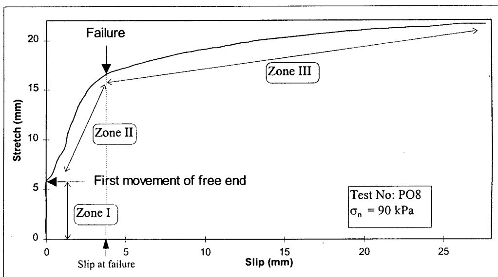
Figure 6-20: Relationship between stretch and slip of the geotextile ( \sigma_n = 90 kPa)
