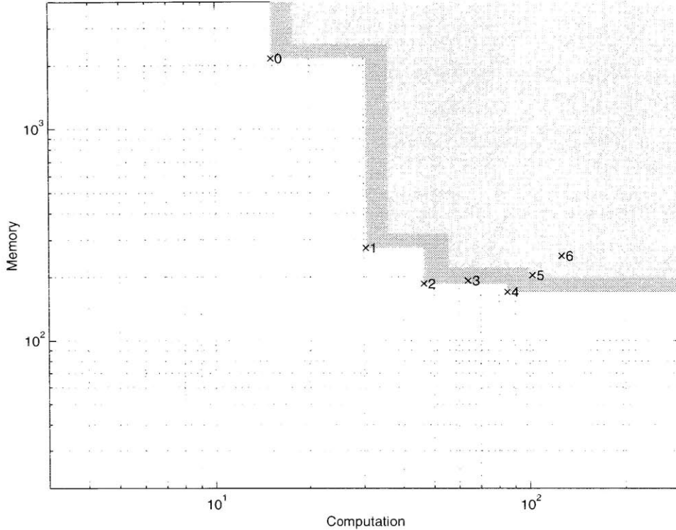
Figure 2-11: Performance plot for the elementary resampler (minimum phase).
