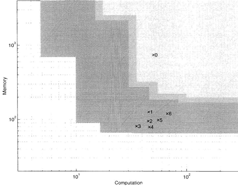
Figure 2-22: Achieved performance when h_D[n] is accounted for (minimum phase).
