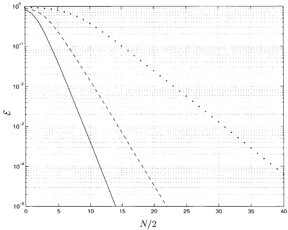
Figure 5-10: \mathcal{E} as a function of N for different \gamma .
