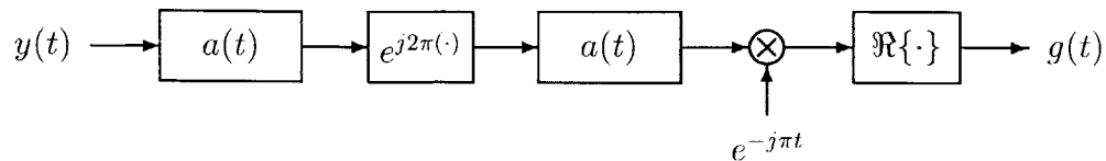
Figure 4-11: Ideal CT system for calculating g(t) .
