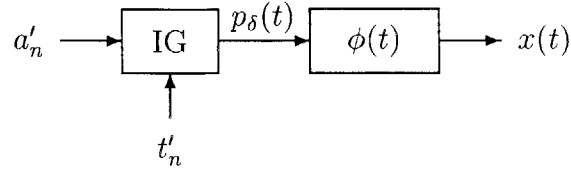
Figure 5-1: Lowpass reconstruction system.
