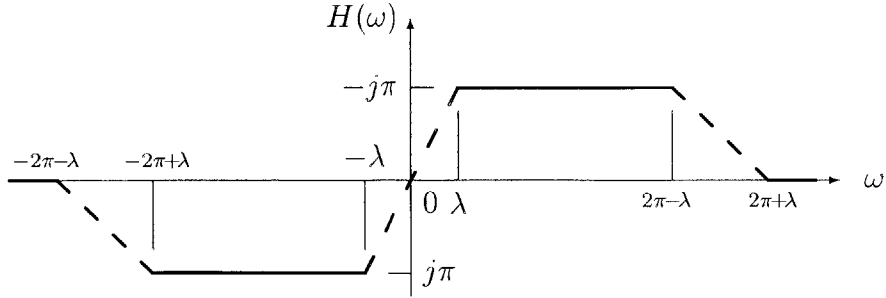
Figure 5-6: Frequency response H(\omega) .
