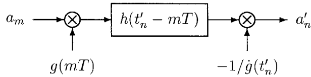
Figure 5-7: Ideal DT resampling system.
