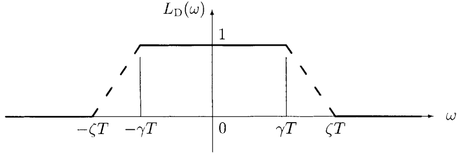
Figure 4-9: Frequency response L_D(\omega) .
