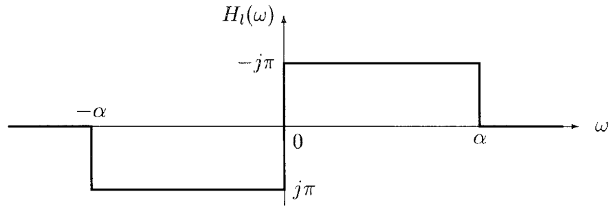
Figure 4-3: Frequency response H_l(\omega) .
