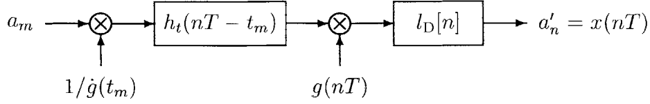
Figure 4-8: Ideal DT resampling system.
