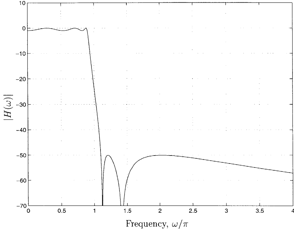
Figure 3-9: The magnitude response of the sixth-order IIR filter.
