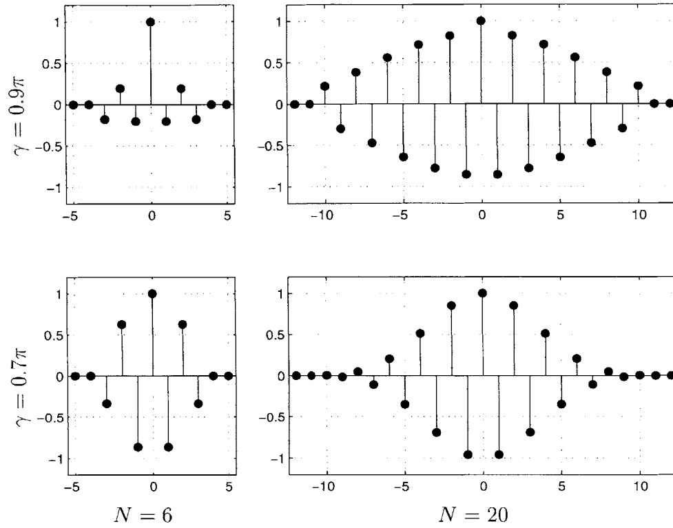
Figure 5-9: Examples of optimal sequences \{b_n\} .
