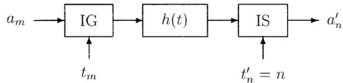
Figure 2-12: Elementary resampler with regular output grid.
