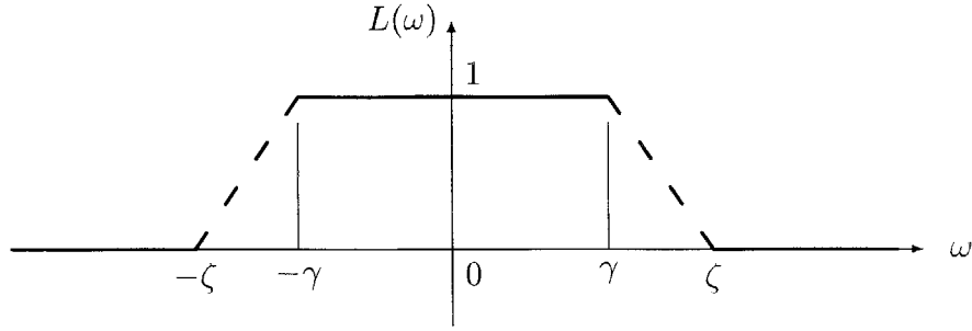
Figure 4-4: Frequency response L(\omega) .
