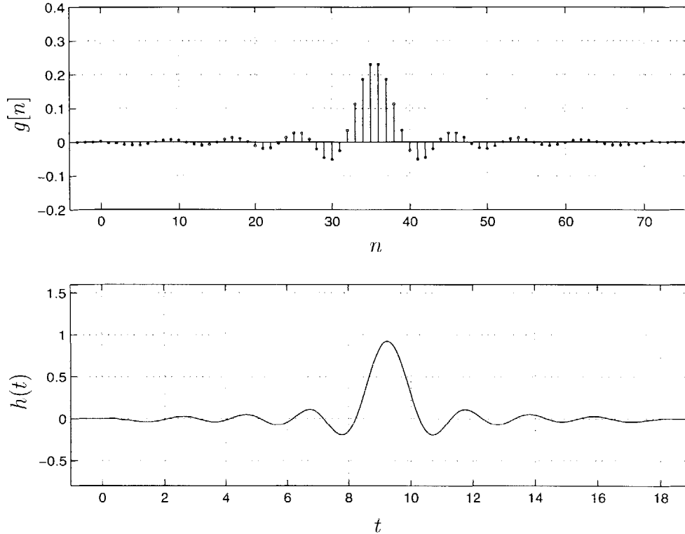
Figure 2-8: The filters g[n] and h(t) . ( k = 2 , linear phase)
