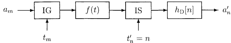
Figure 2-13: Elementary resampler with a fixed DT filter.
