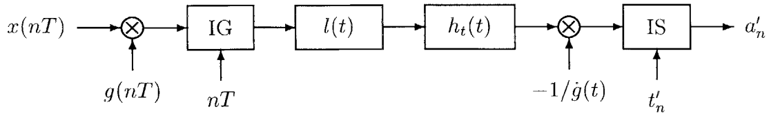
Figure 5-4: System with discrete input and output.
