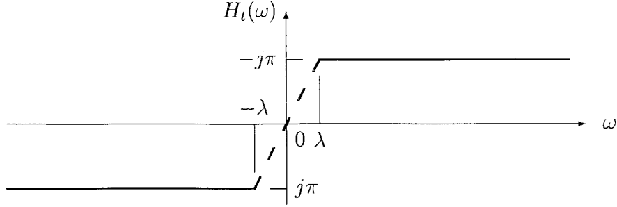
Figure 5-3: Frequency response H_t(\omega) .
