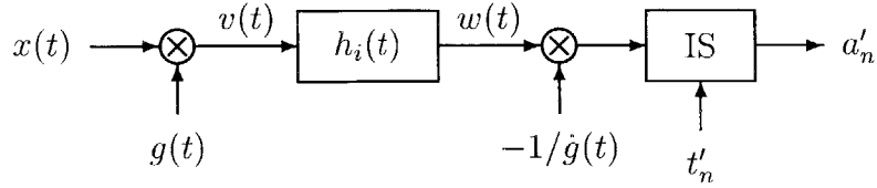
Figure 5-2: Ideal CT system.
