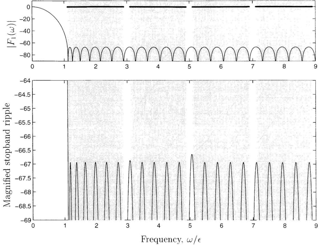
Figure 2-14: Frequency response |F_1(\omega)| , and magnified stopband.
