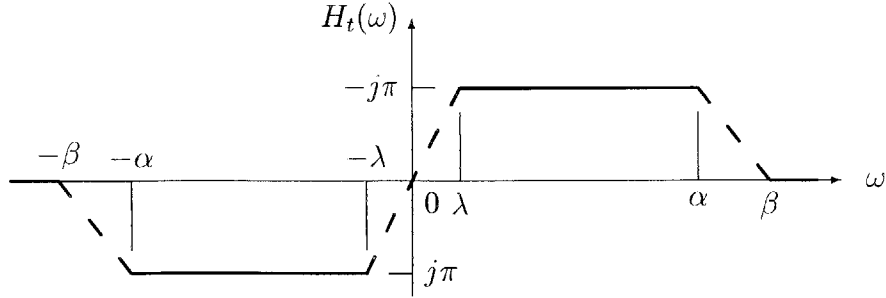
Figure 4-6: Frequency response H_t(\omega) .
