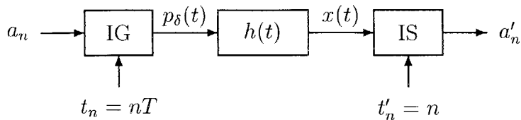
Figure 3-1: Generic sampling rate converter.
