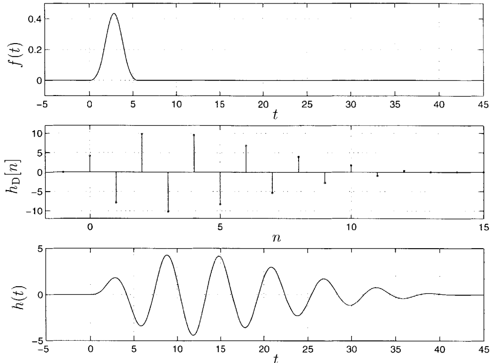
Figure 2-18: Filters f(t) , h_D[n] and h(t) ( k = 3 , minimum phase).
