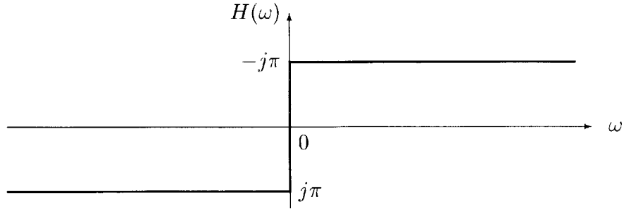
Figure 4-2: Frequency response H(\omega) .
