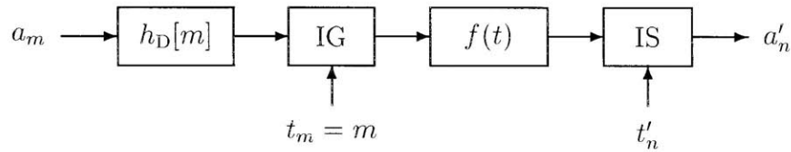
Figure 2-23: Elementary resampler with regular input grid.
