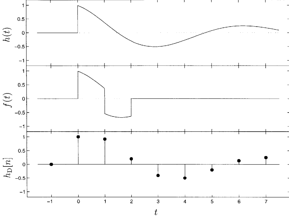
Figure 3-5: f(t) , h_D[n] and the equivalent filter h(t) (second order case).
