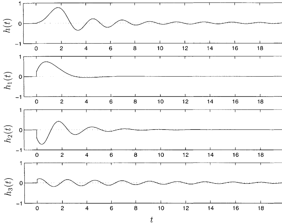
Figure 3-6: Sixth-order IIR filter and its three second-order components.
