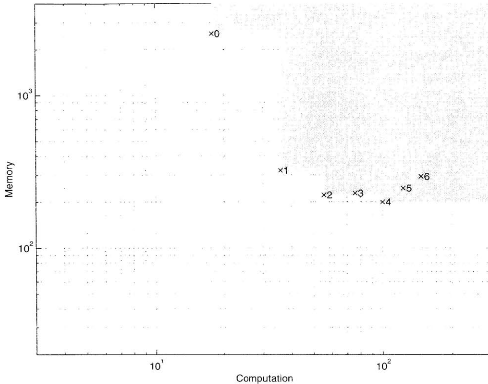
Figure 2-10: Performance plot for the elementary resampler (linear phase).
