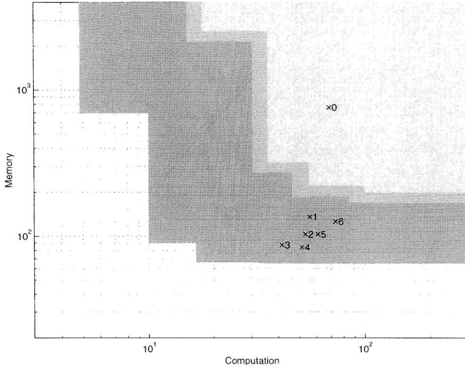
Figure 2-21: Achieved performance when h_D[n] is accounted for (linear phase).
