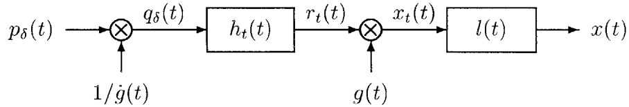
Figure 4-7: Reconstruction system which allows transition bands.
