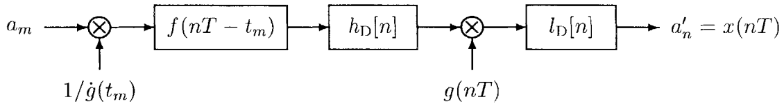
Figure 4-10: DT system which allows for a short time-varying filter.
