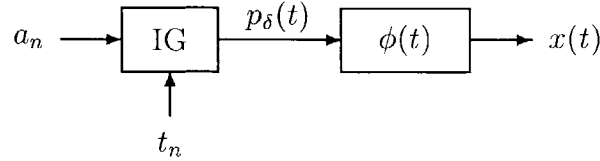
Figure 1-1: The ideal lowpass reconstruction system.
