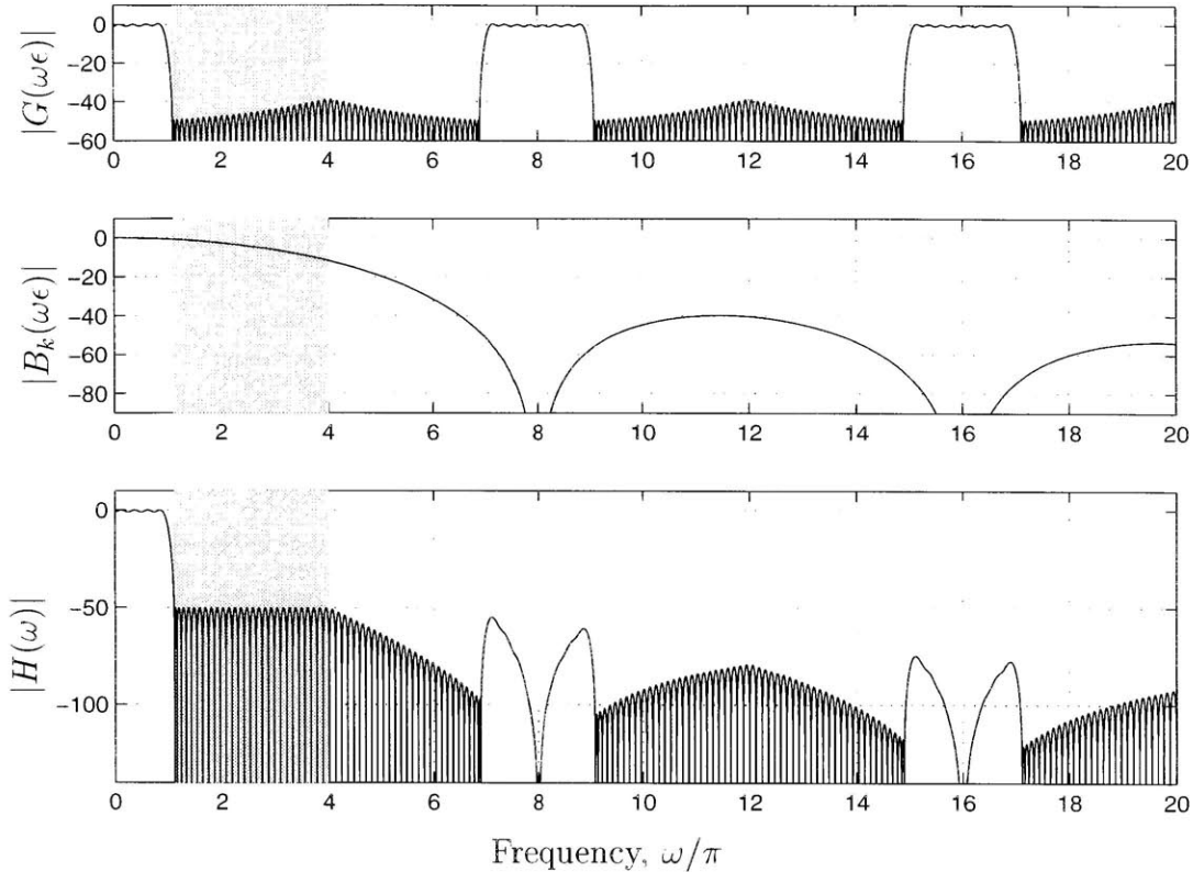
Figure 2-7: |H(\omega)| and its factors |G(\omega\epsilon)| and |B_k(\omega\epsilon)| .
