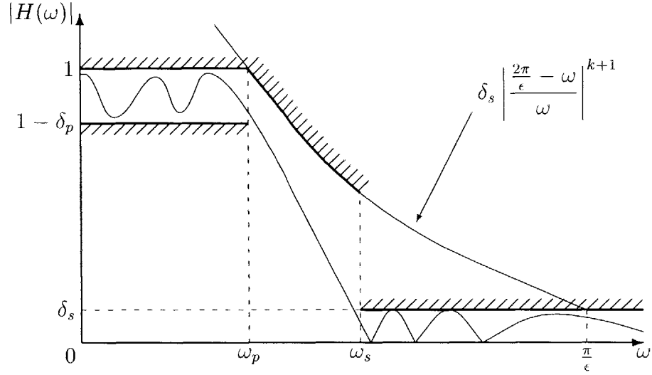
Figure 2-6: Filter specification with an additional constraint.
