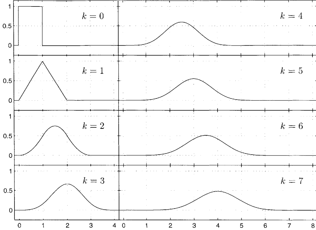
Figure 2-3: The first eight non-centered B-splines.
