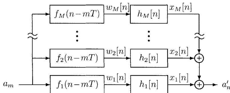
Figure 3-8: Final system for high-quality sampling rate conversion.
