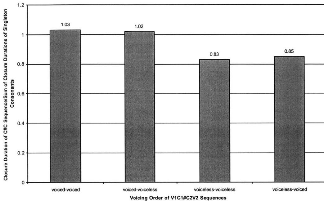
Figure 10. Closure Duration Ratio vs. Voicing Characteristics. A plot of the average ratio of the consonant-sequence closure duration to the sum of the closure durations of singleton C1 and C2 with respect to the order of voicing.
