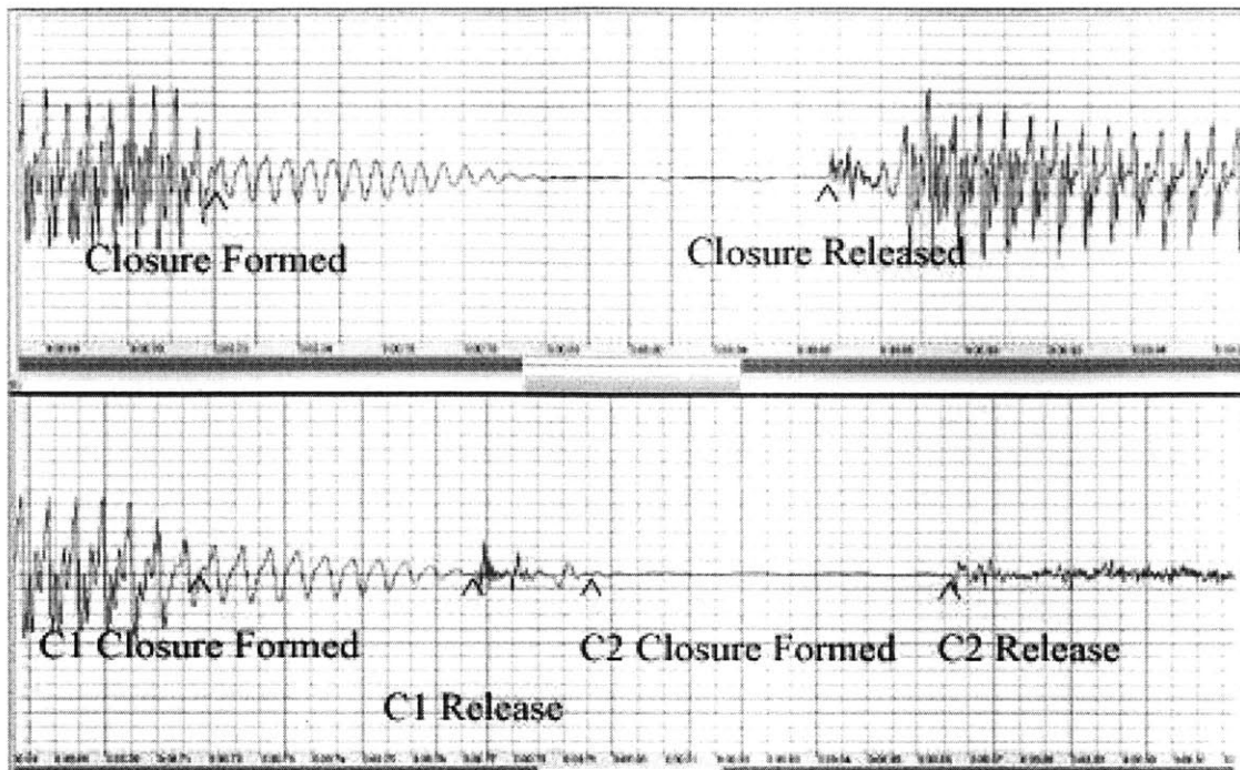
Figure 5. Closure Duration Measurements. The top panel shows how closure duration was measured for VCV sequences. The bottom panel shows how closure durations were measured for VCCV sequences, for cases where C1-bursts were present.
