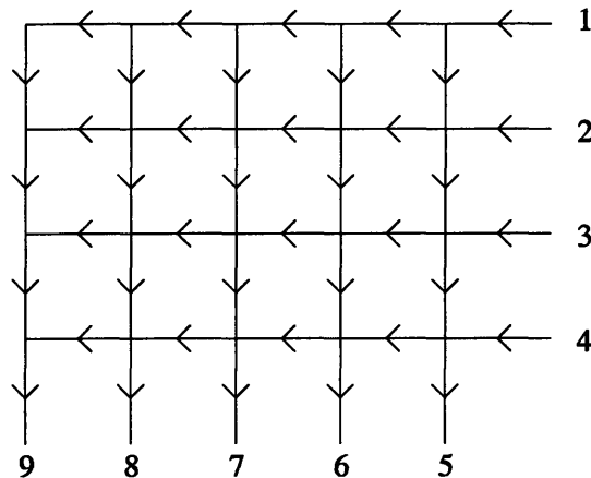
Figure 3-1: \text{Web}_{k,n} for k = 4 and n = 9
