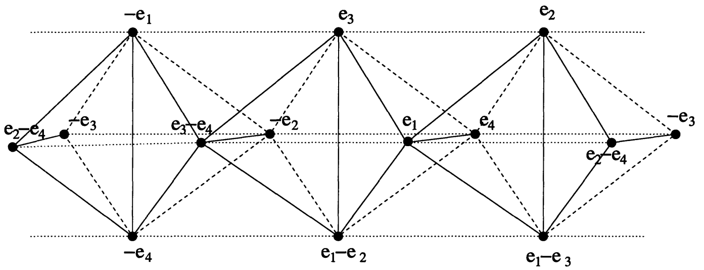
Figure 3-8: The intersection of F_{3,6} with a sphere
