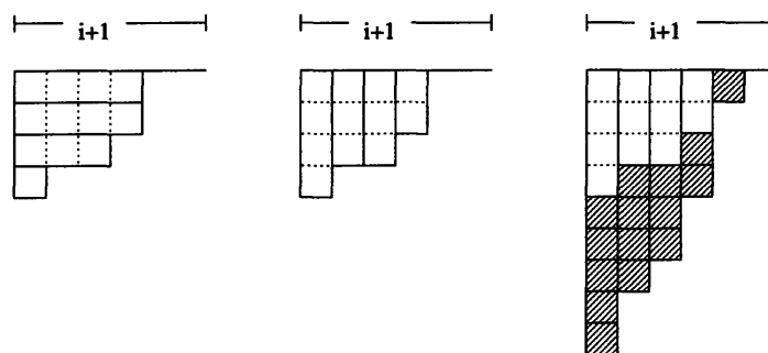
Figure 2-9: A combinatorial interpretation for y^i q^{\binom{i+1}{2}} \prod_{r=1}^{i+1} \frac{1}{1-q^r y}
