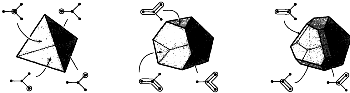
Figure 5-1: P(D_4) ©Satyan Devadoss
