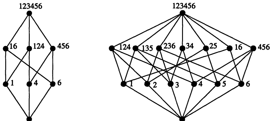
Figure 4-4: The lattice of positive flats and the lattice of flats.
