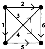
Figure 4-1: The digraph D
