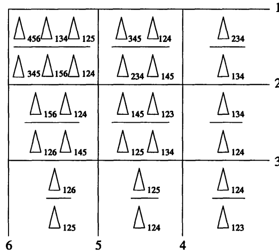
Figure 3-3: \text{Web}_{3,6}
