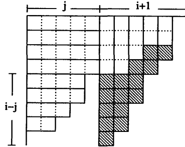
Figure 2-10: (\lambda, \hat{\lambda}) , where \lambda = (5, 5, 5, 5, 4, 4, 3, 2, 0) and \hat{\lambda} = (9, 8, 6, 4, 3, 0)
