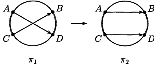
Figure 2-6: Covering relation
