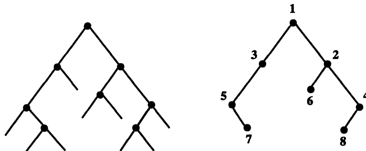
Figure 4-7: A type \tau tree and an increasing binary tree of type \tau' .
