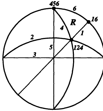
Figure 5-3: The braid arrangement A_3 .
