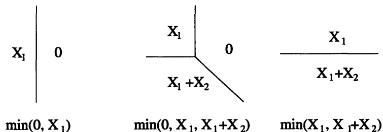
Figure 3-5: Fans for \text{Trop } P_J
