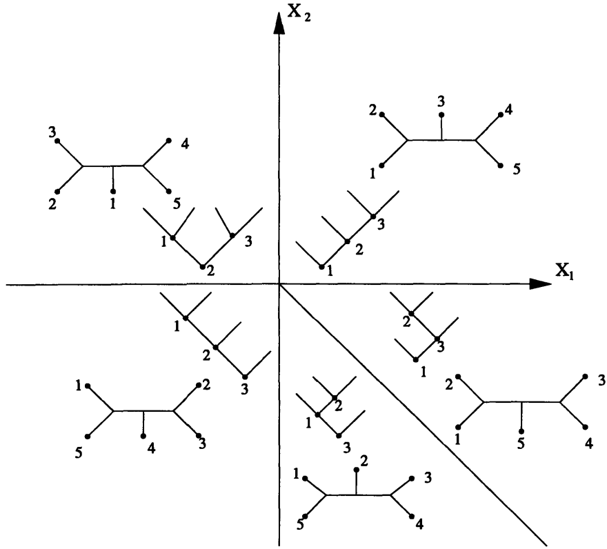
Figure 3-6: The fan of \text{Trop}^+ Gr_{2,5}
