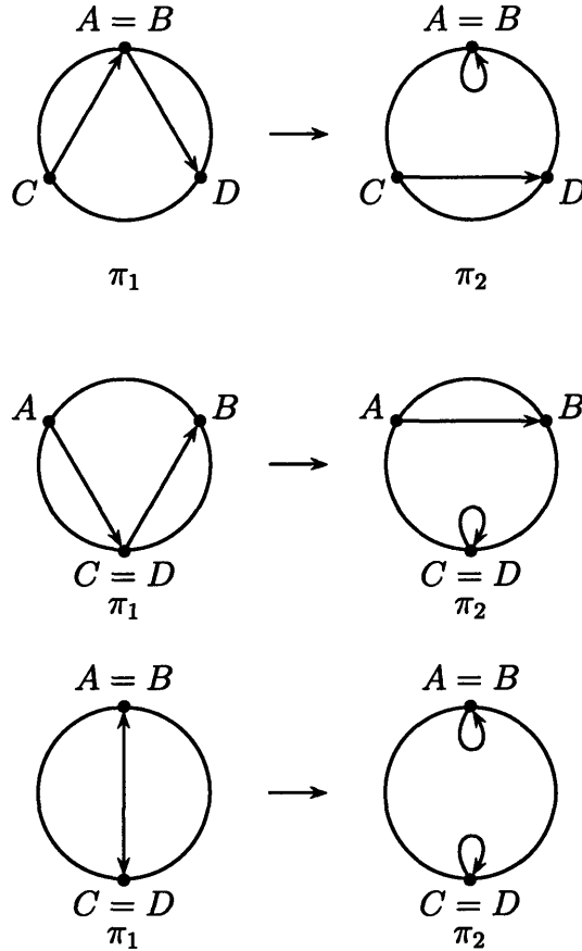
Figure 2-7: Degenerate covering relations
