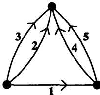
Figure 4-3: The digraph D' .
