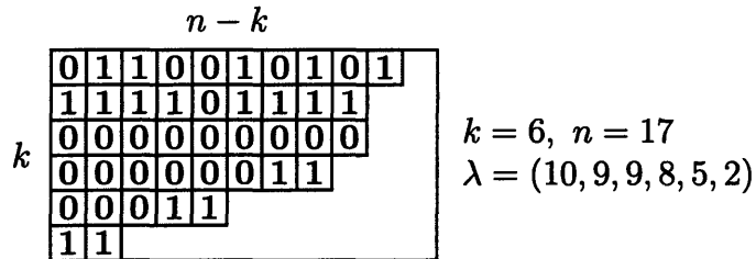
Figure 2-2: A \mathcal{J} -diagram (\lambda, D)_{k,n}
