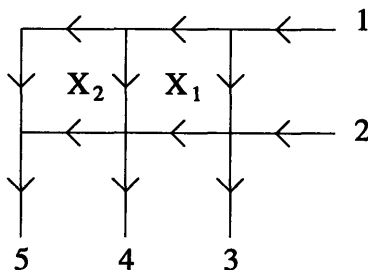
Figure 3-4: \text{Web}_{2,5}
