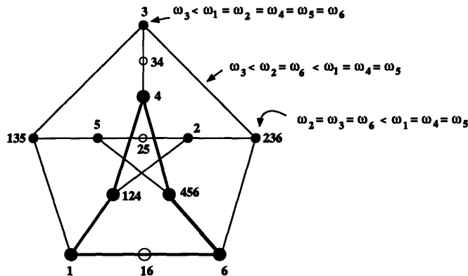
Figure 4-6: \mathcal{B}^+(K_4) \subset \mathcal{B}(K_4)
