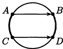
Figure 2-4: A crossing
