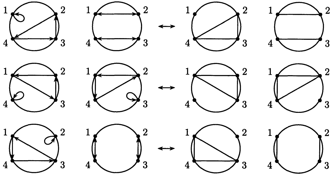
Figure 2-11: The bijection between maximal-alignment permutations and noncrossing partitions
