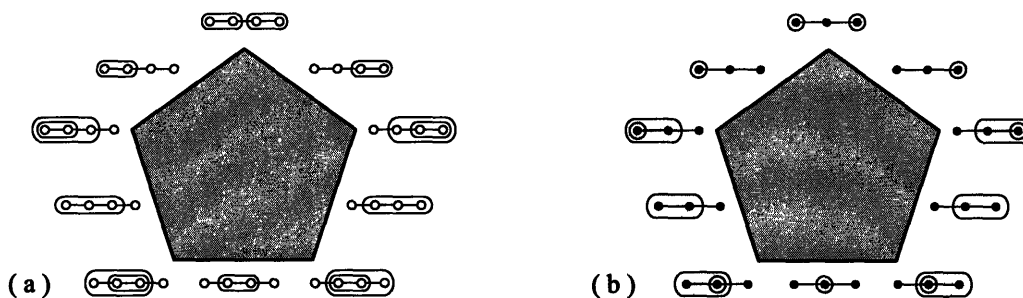
Figure 5-2: A_2 is P(A_3) ©Satyan Devadoss
