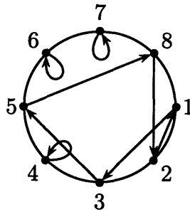
Figure 2-3: A chord diagram for a decorated permutation
