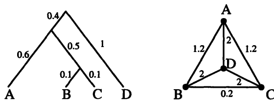
Figure 4-5: An equidistant tree and its corresponding distance vector.
